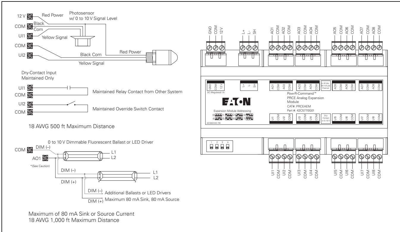
Figure 235-9. PRCE Analog Expansion Module I/O Connections
