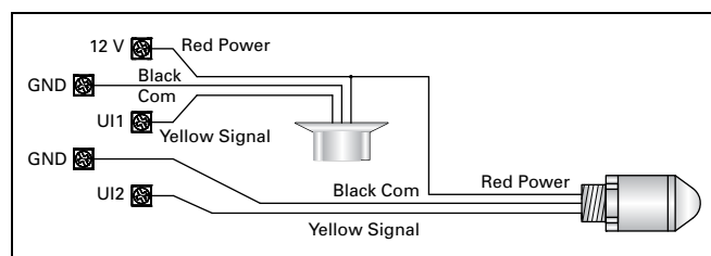
Figure 23.5-7. Photosensor Connection
