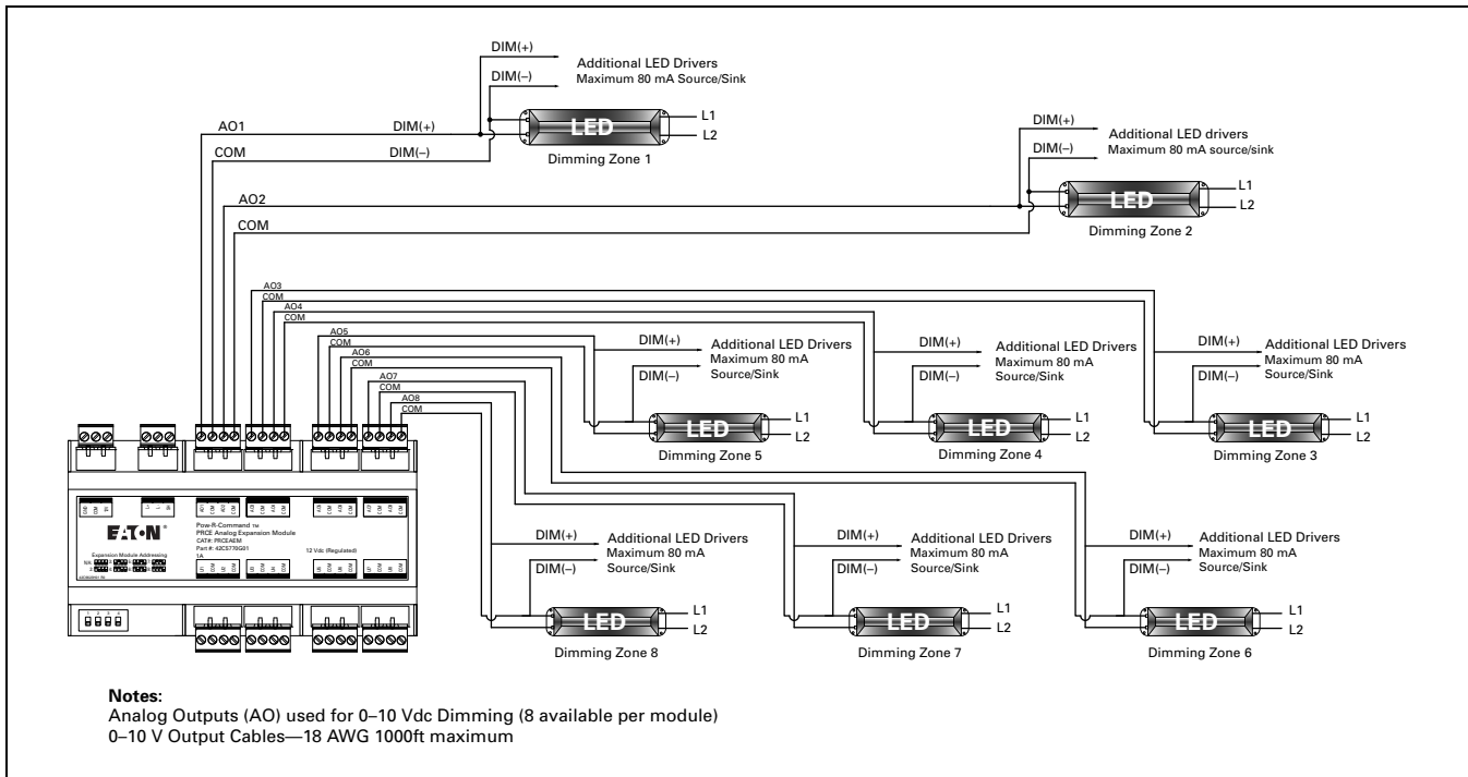
Figure 235-10. PRCE Analog Expansion Module 0–10 Vdc Dimming Outputs
