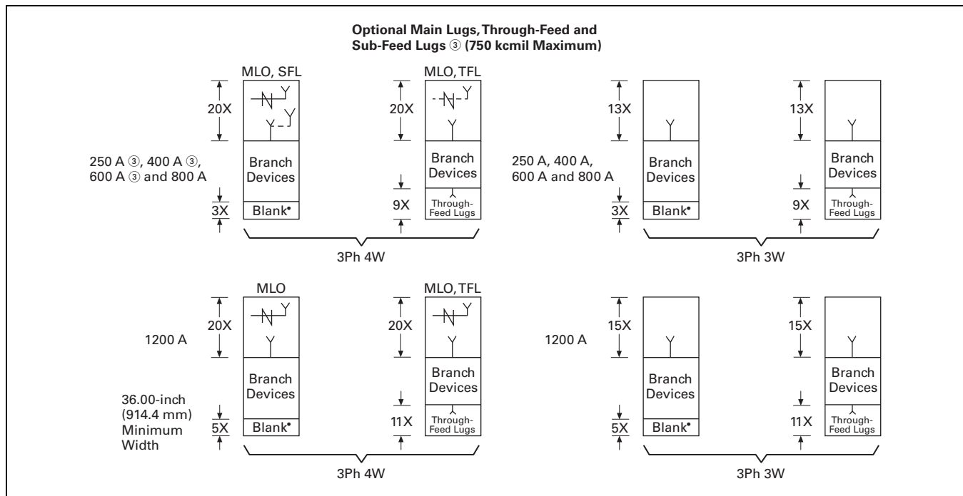
Figure 22.4-5. "X" Space Requirements—Dimensions in Inches (mm)
