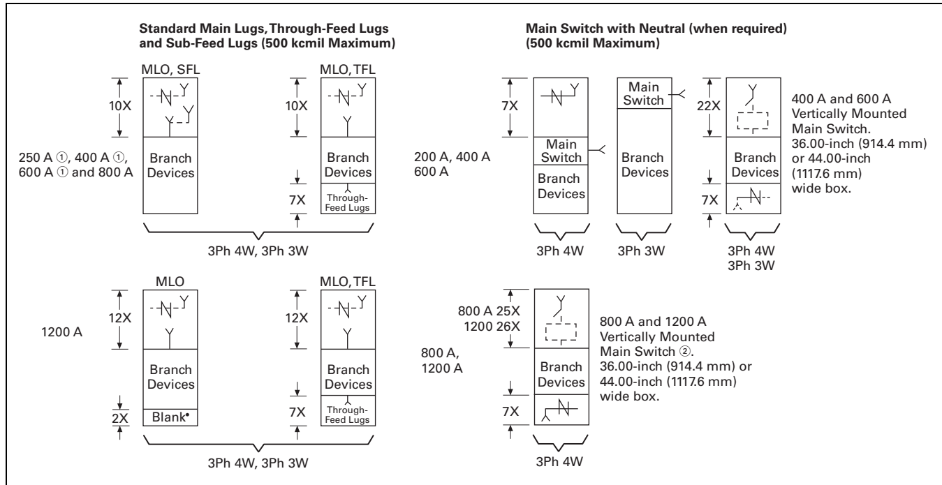
Figure 22.4-4. "X" Space Requirements—Dimensions in Inches (mm)
