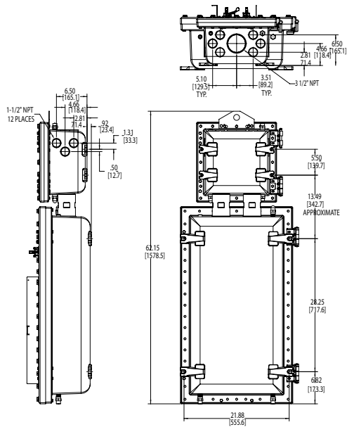
Size C and D Panel (with cast aluminum terminal housing)
