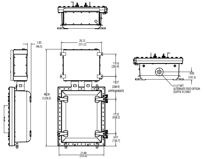
Size B Panel (with stainless steel terminal housing)
