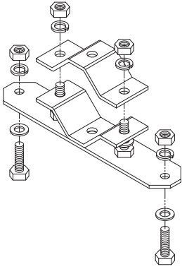
FPSPMKIT 1-1/4" pole mount
