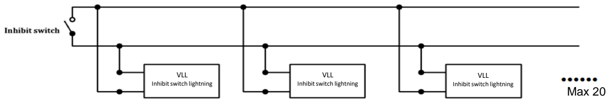
Wiring diagram 3: Inhibit switch light fitting External connection
