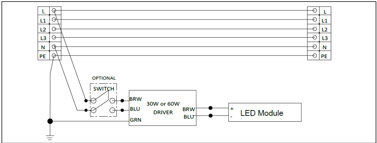
Wiring diagram 1: 2 feet or 4 feet normal version
