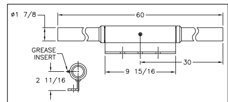
Crane Boom Mount Dimensions
