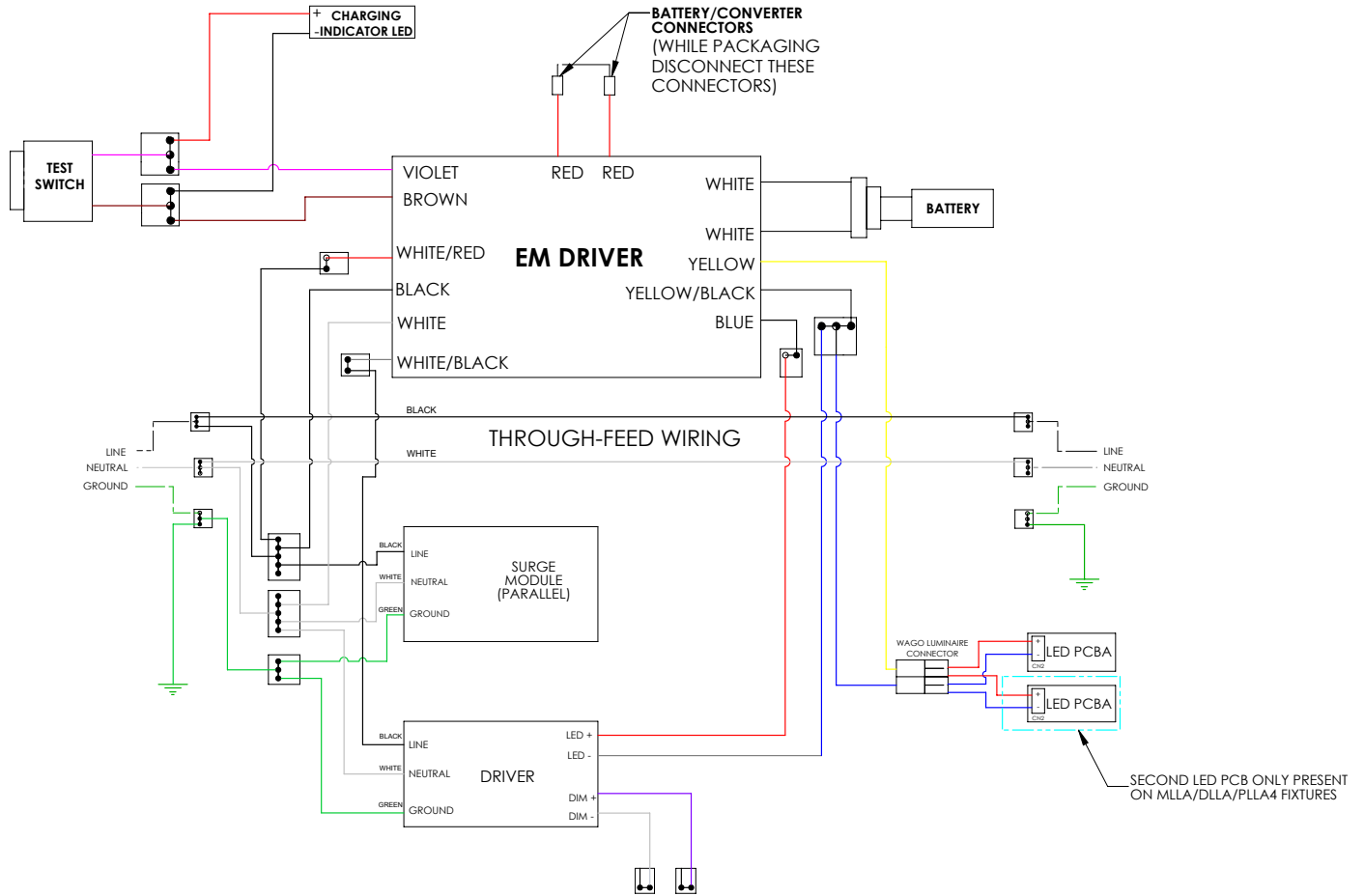
Figure 5: MLLA/DLLA/PLLA EM M2 Surge Option System Wiring Diagram
