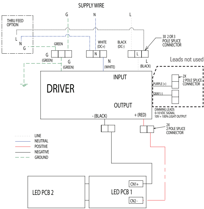
2 Foot UNV1 Wiring Diagram - Figure 15A
