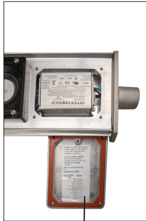
Driver Cover
