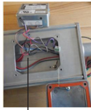
Wire Channel
