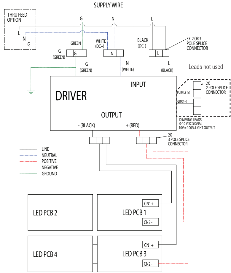
4 Foot UNV1 Wiring Diagram - Figure 15B
