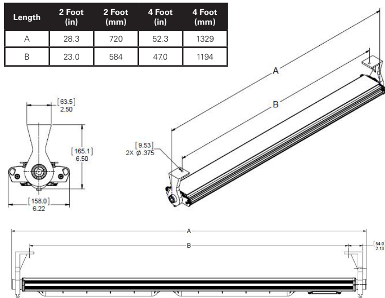
Figure 2. DP1053MTK Wall/Ceiling Mount Installation
