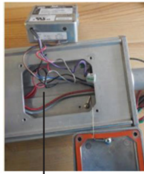
Wire Channel
