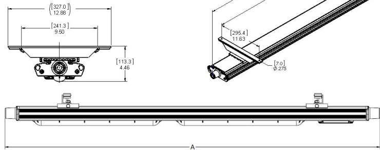
Figure 6. MP1054MTK Kit MagnaPro Mount Kit Installation
