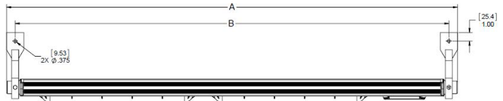
Figure 1. DP1052MTK Side Mount Installation
