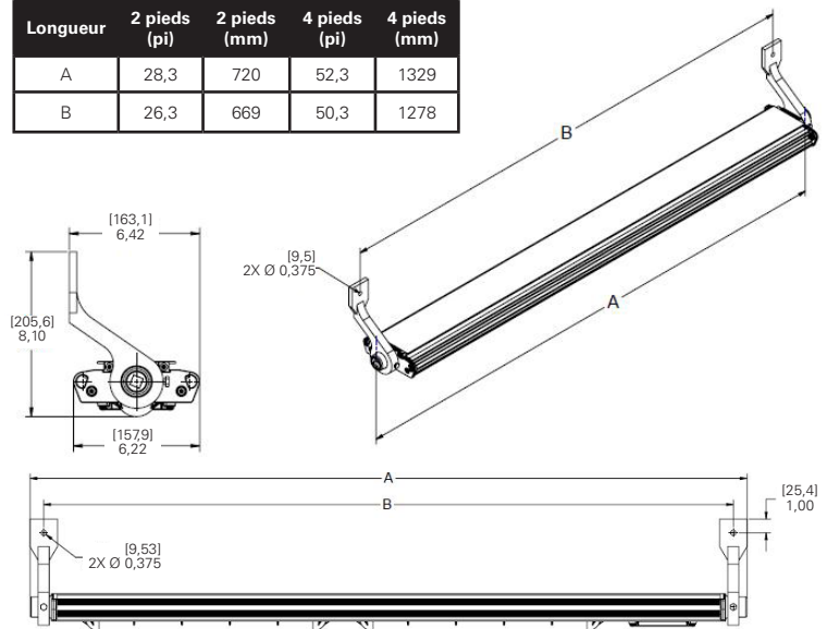
Figure 1 : Montage mural DP1052MTK
