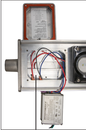
Wire Channel
