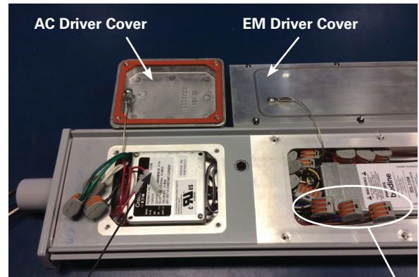
Battery/Converter Connector
