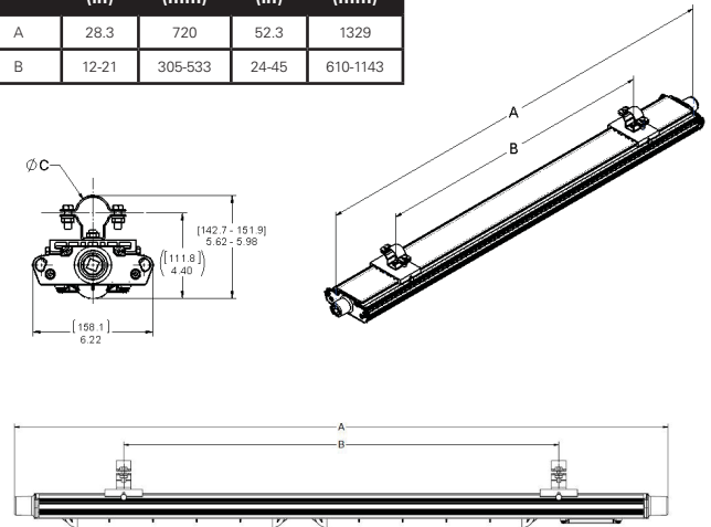
Figure 8. PM KIT - Pole Mount Installation
