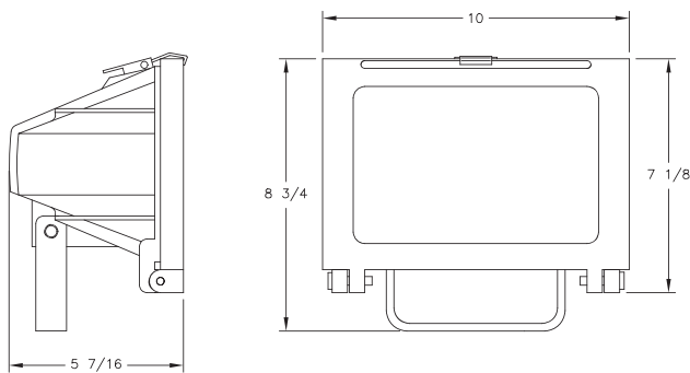
QA-L trunnion mount
