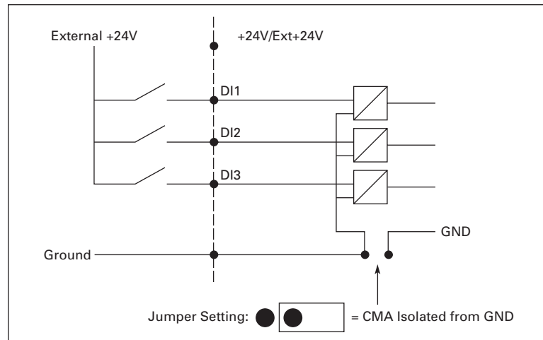
Figure 1-4: Positive Logic
