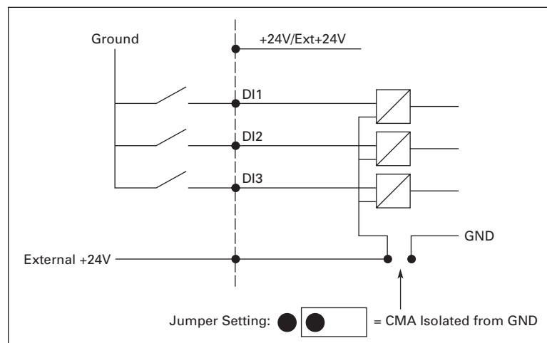
Figure 1-5: Negative Logic
