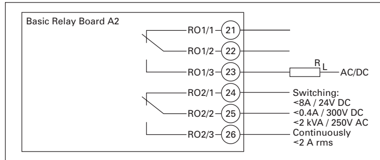
Figure 3-4: Option Board A2 Wiring Diagram
