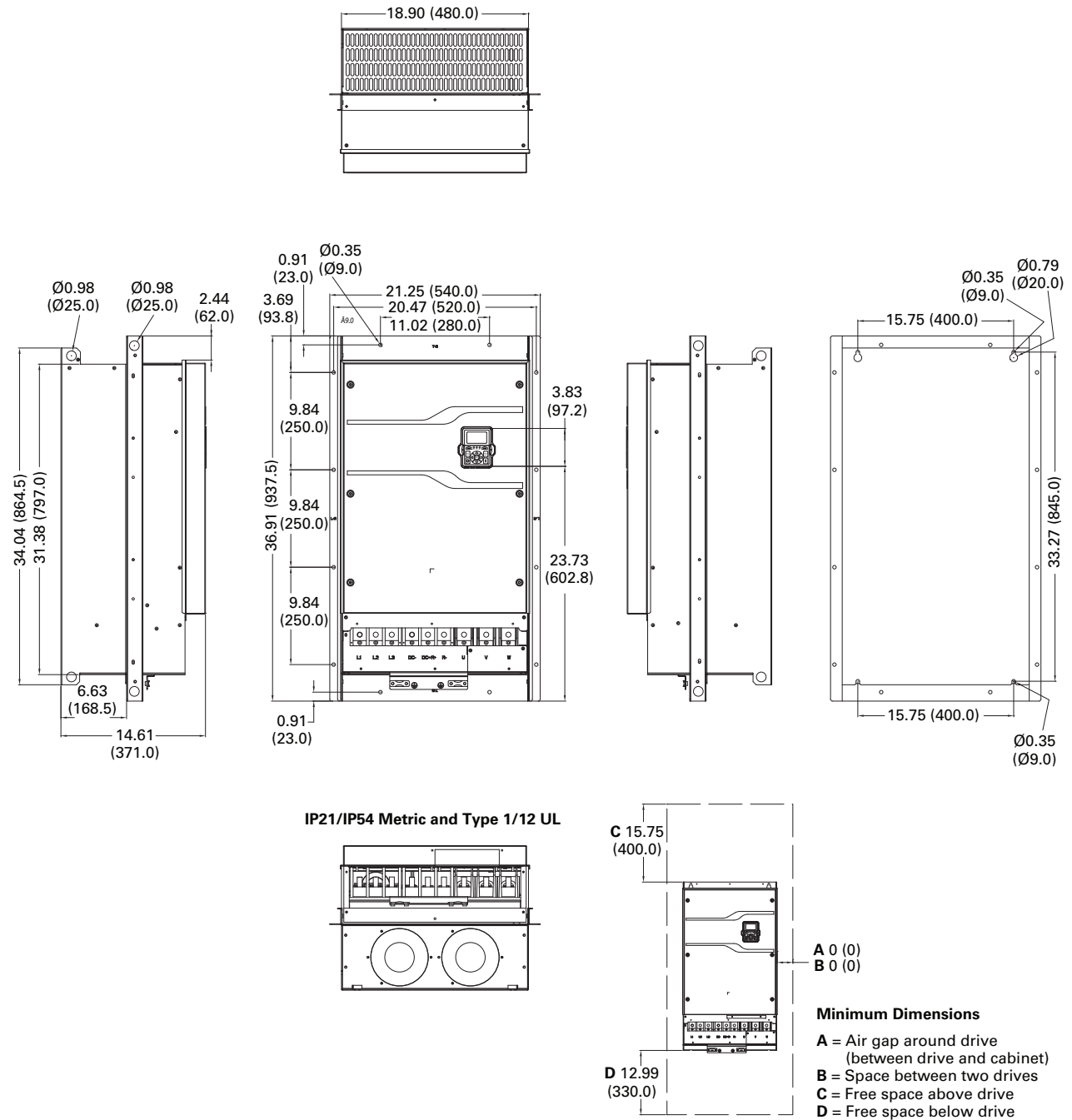
Figure 52. FR6 Dimensional drawing flange mount
