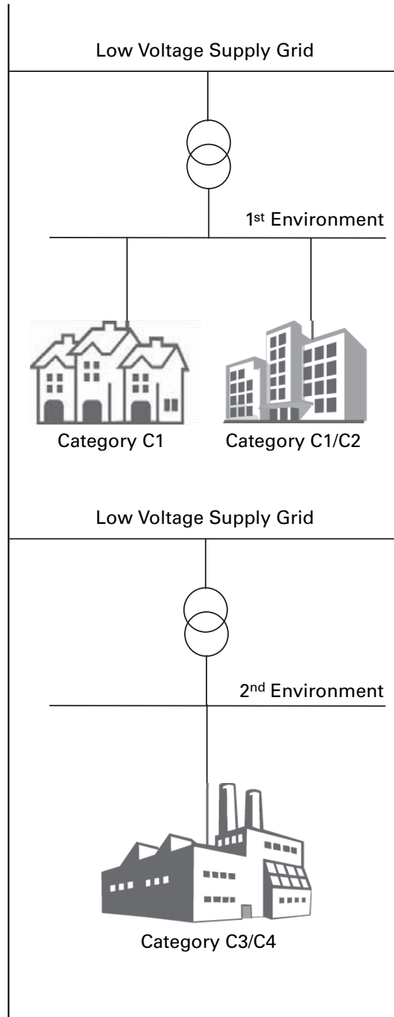
Figure 13. EMC Measures
