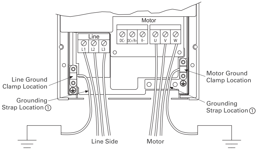
Figure 24. Ground wiring
