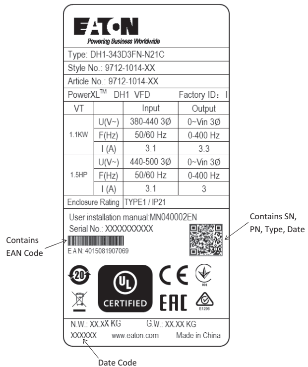
Figure 5. Carton label—DH1
