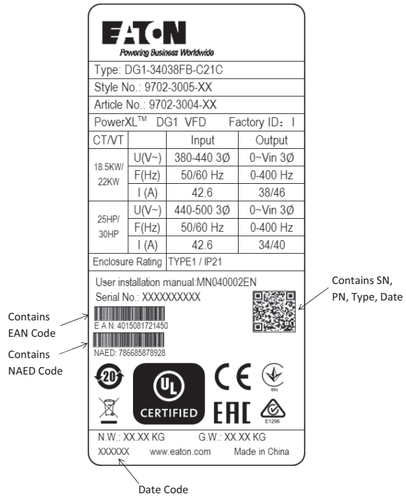
Figure 4. Carton label—DG1
