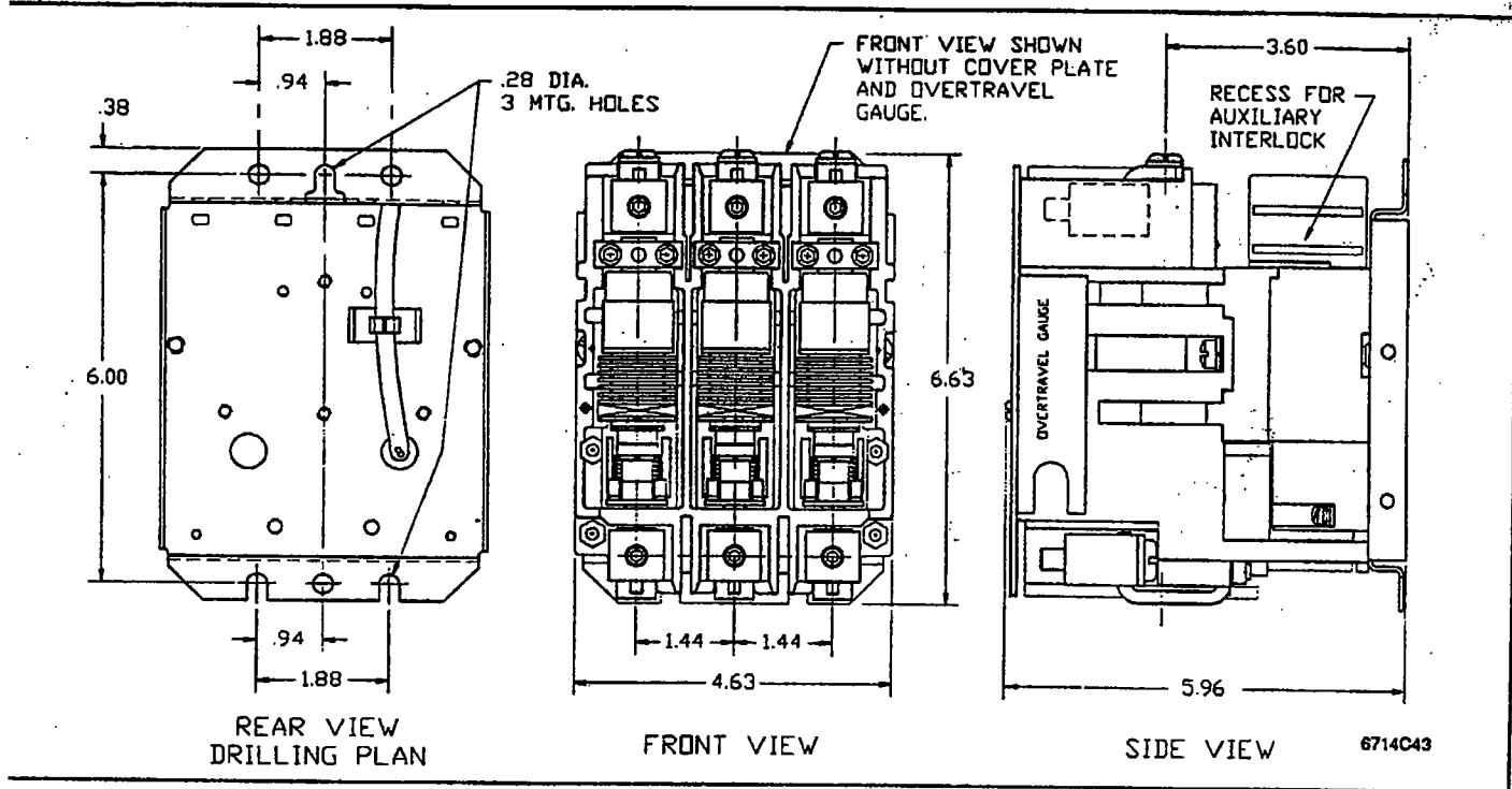
Fig. 8 Nonreversing Contactor (V201) Dimension Drawing (Dimensions in inches)
