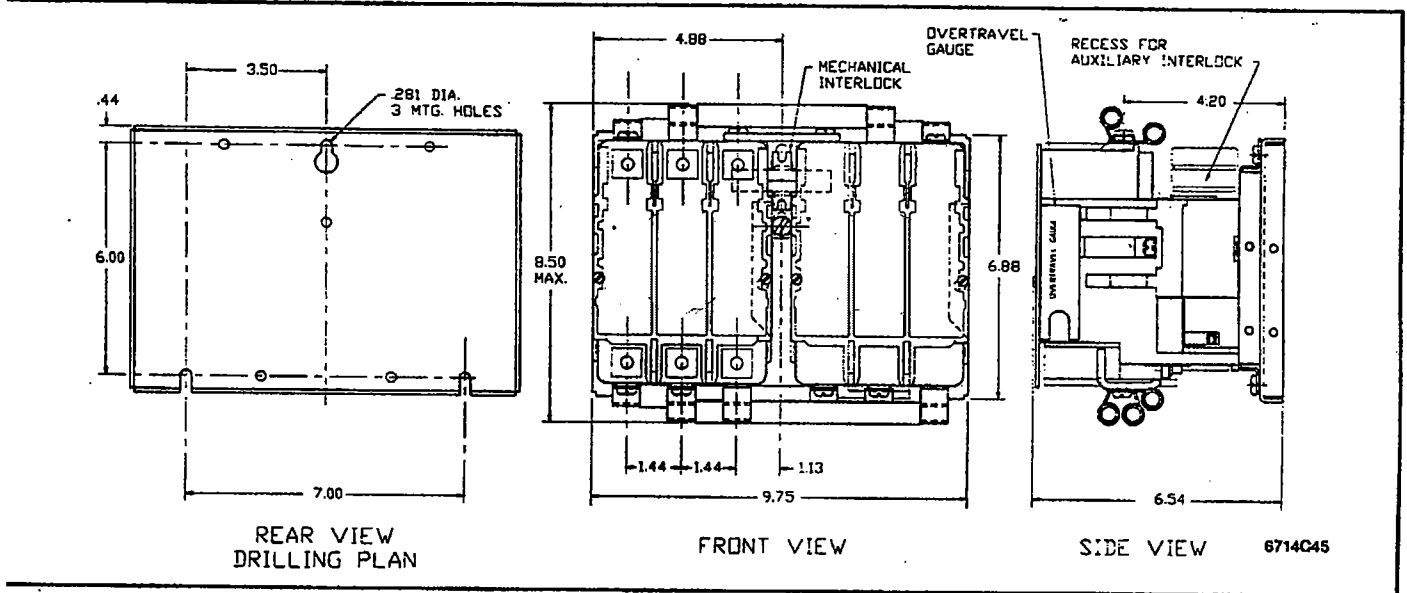
Fig. 9 Reversing Contactor (V211) Dimension Drawing (Dimensions in inches)
