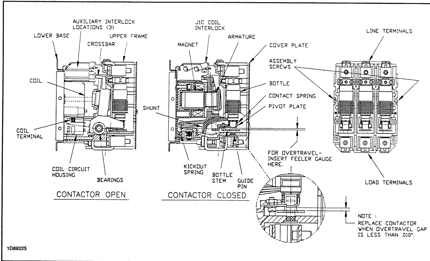
Fig. 3 Size 4 Vacuum Contactor
