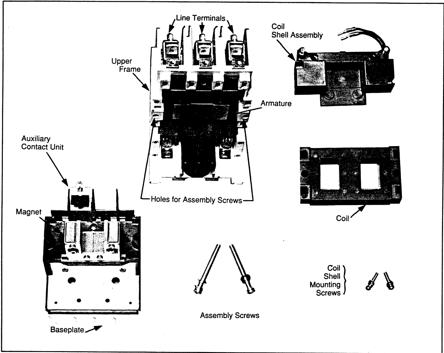
Fig. 4 Size 4 Vacuum Contactor Disassembled
