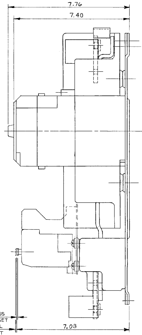
TITLE DIMENSIONS FOR SIZE "S" STARTER
