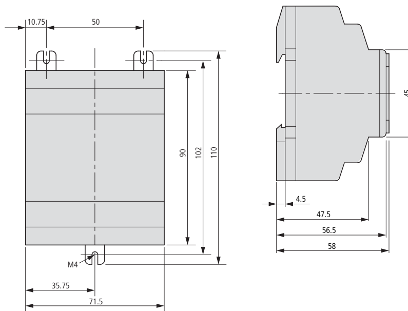
Figure 104: Dimensions of easy512-... in mm (for dimensions in inches see table 36)
