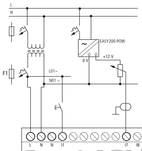
Figure 20: easy-AB analog input, connection of reference potentials
