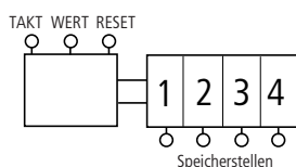
Figure 85: Block diagram of the 4-way shift register
