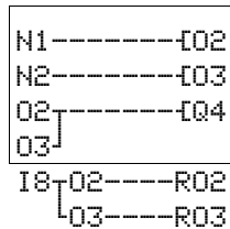
Circuit diagram display
