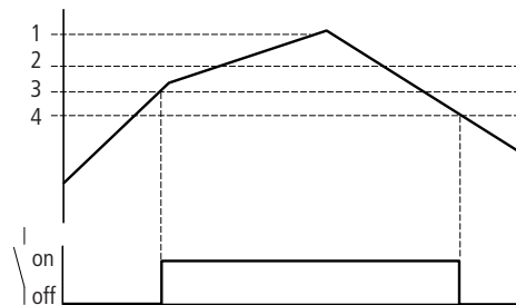
Figure 52: Signal diagram of analog value comparator in Greater than/equal to mode
