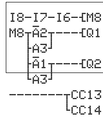
Circuit diagram display
