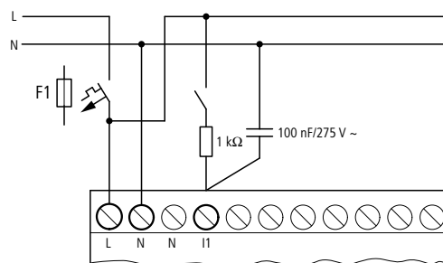
Figure 16: Limitation of the input current through resistors
