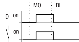
Figure 61: Night switching signal diagram
