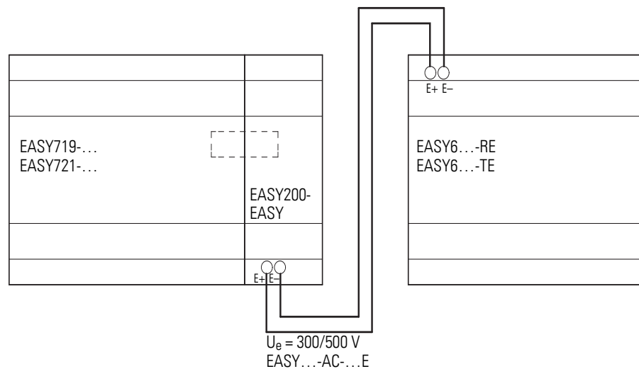
Figure 36: Connecting remote expansion units to easy
