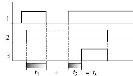
Figure 73: Function of the circuit
