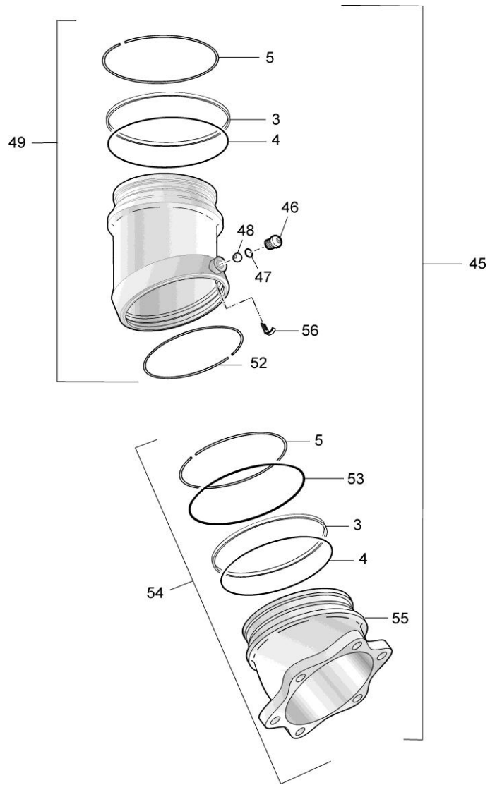
FIGURE 8 47566 SWIVEL ELBOW INLET COUPLING - OPTION N
