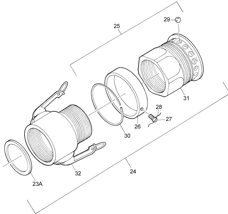
FIGURE 4 44771 Inlet – Option S
