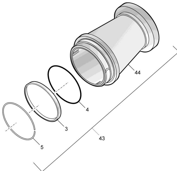
FIGURE 7 47063 INLET - OPTION W
