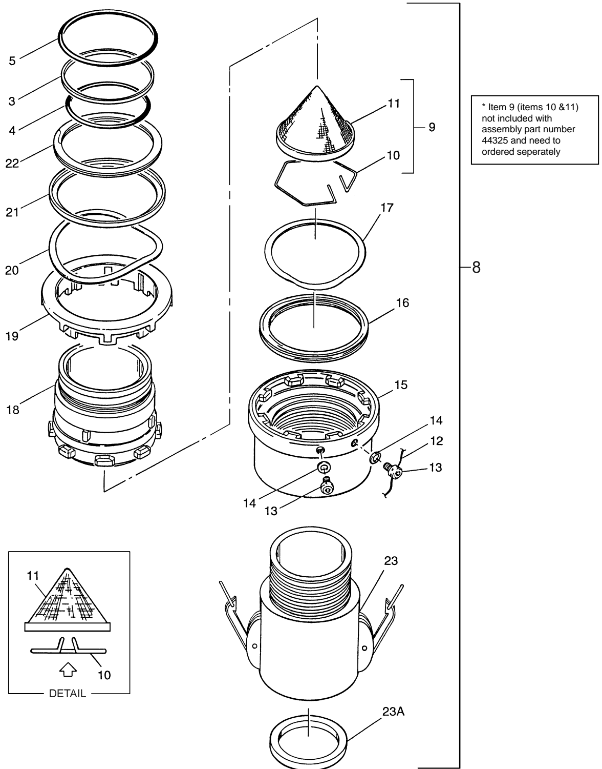
FIGURE 3 44325 INLET – OPTION K
