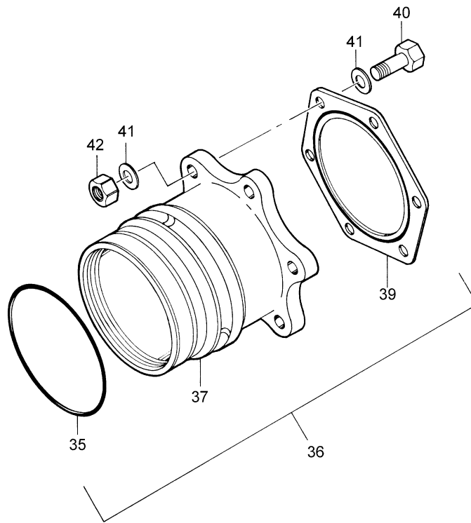
FIGURE 6 43045-1 ADAPTER - OPTION 2
