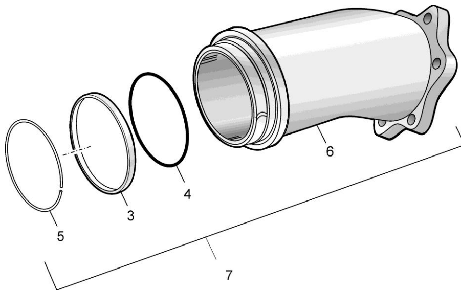
FIGURE 2 44327 D-1 INLET – OPTION H
