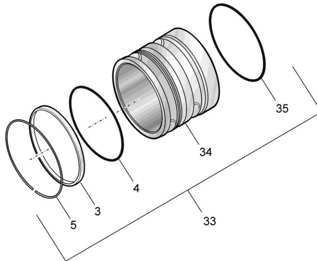
FIGURE 5 44362 ADAPTER – OPTION 9
