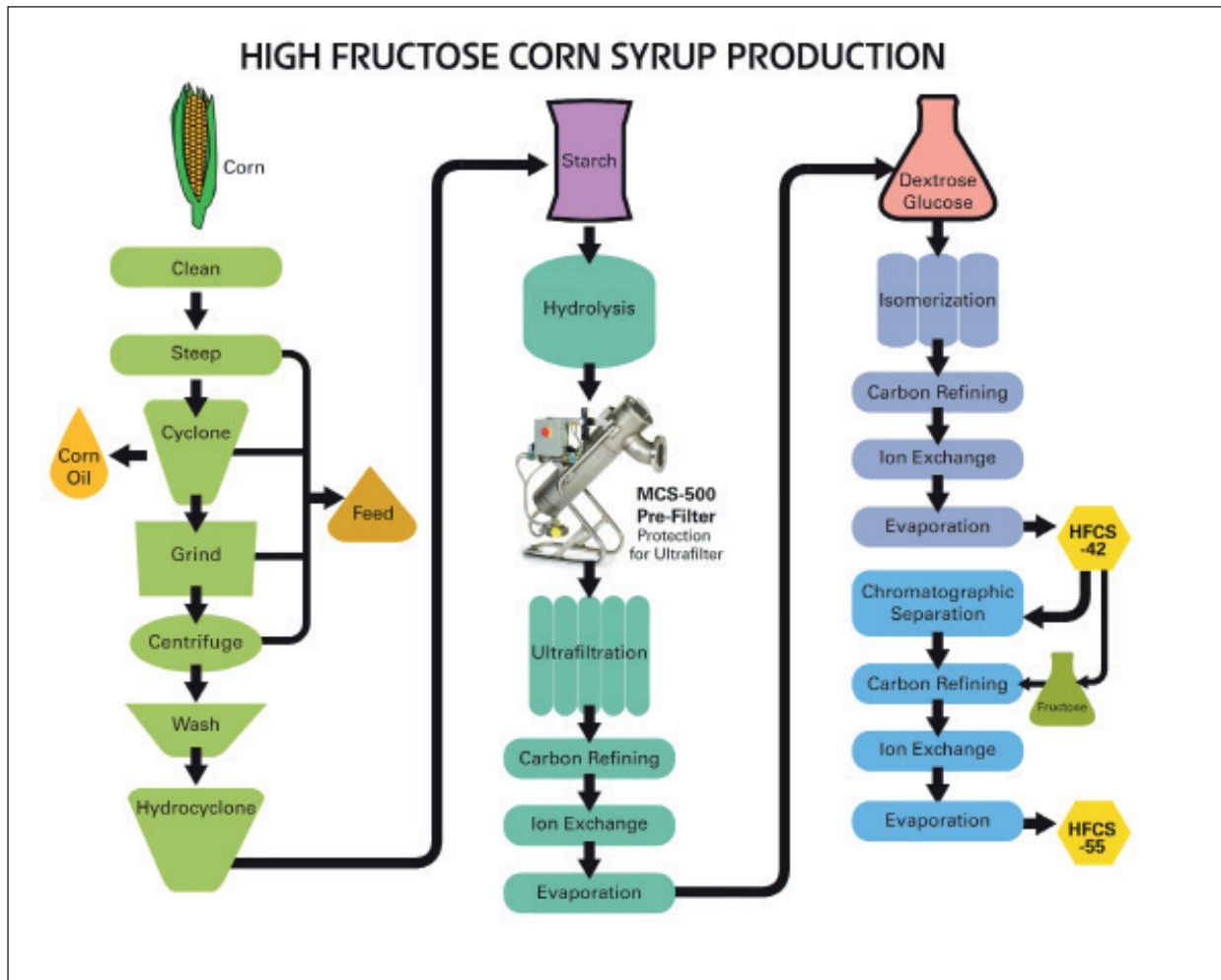
Corn syrup production process chart.
