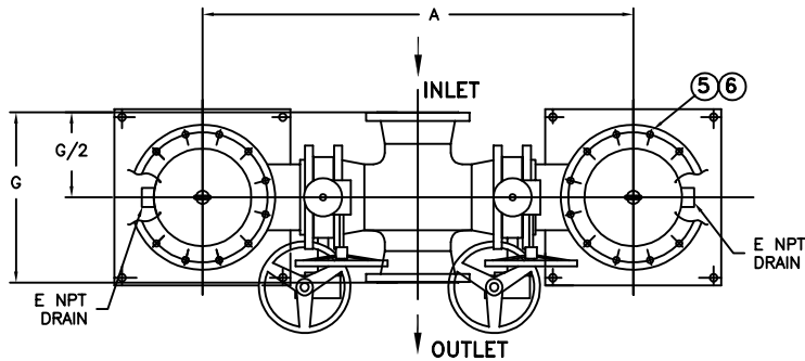
ASSEMBLY PLAN VIEW
