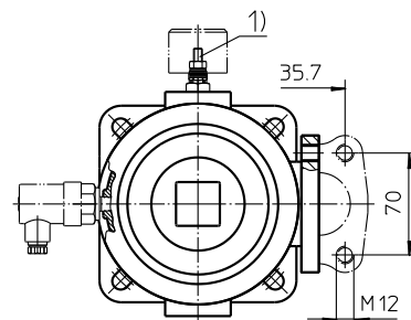
SAE-connection
