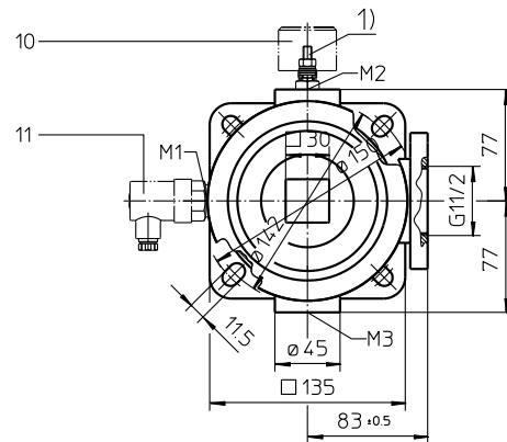
thread connection
