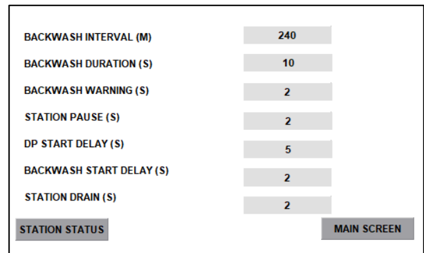
Image 4: Display showing External Backwash Parameters
