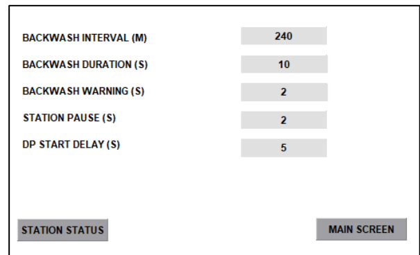
Image 3: Display showing Internal Backwash Parameters
