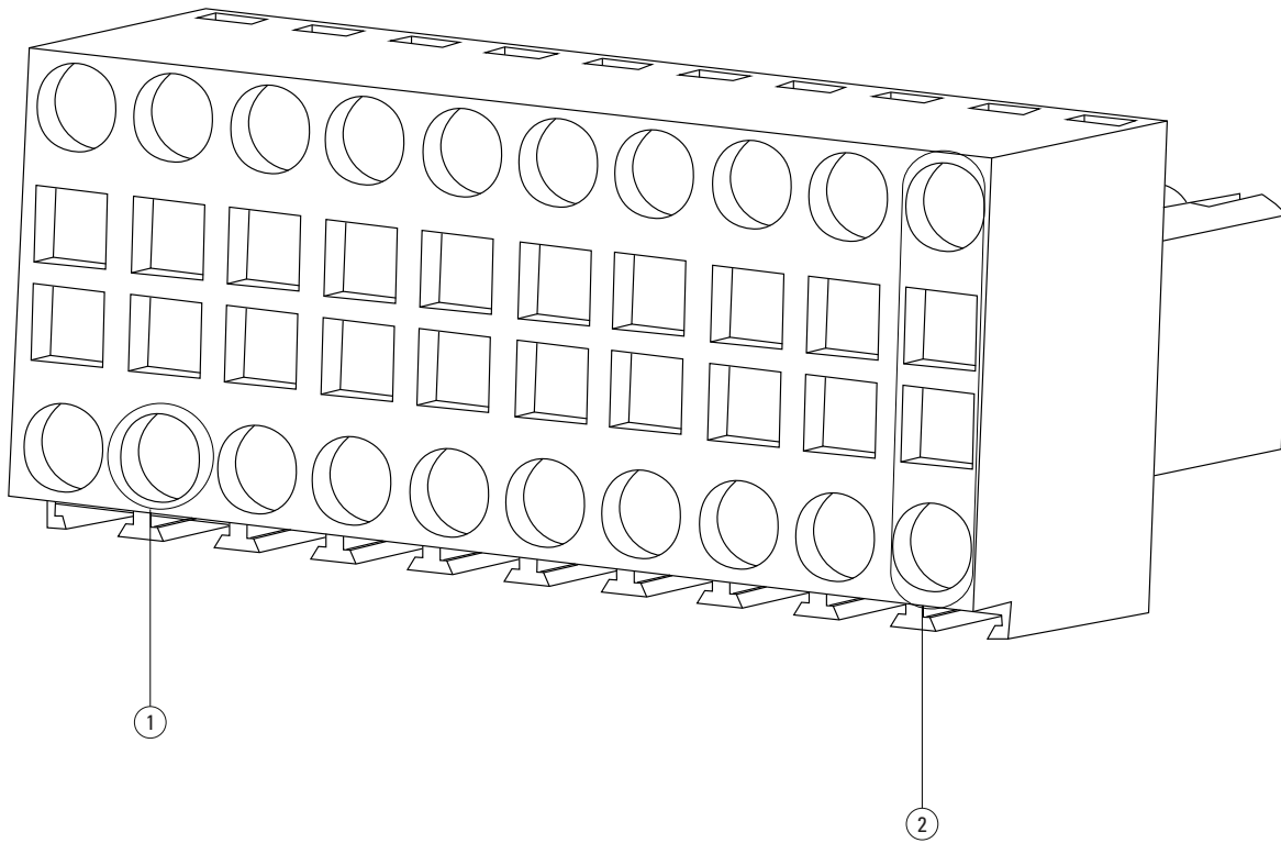
Figure 13. J9 mating connector
