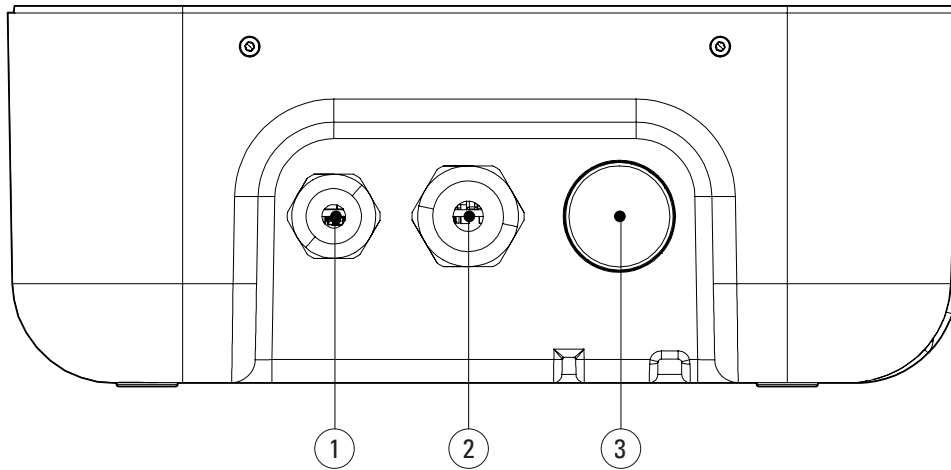
Figure 17. Bottom view of the Green Motion Home EV charger
