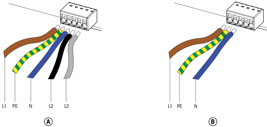
Figure 10. How to wire AC distribution grid wires to the power supply terminal of the Green Motion Home EV charger
