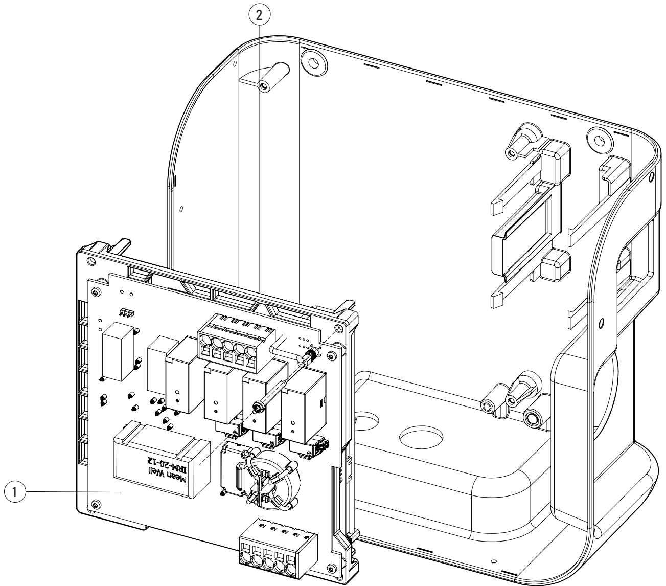
Figure 14. Location of the AC platform
