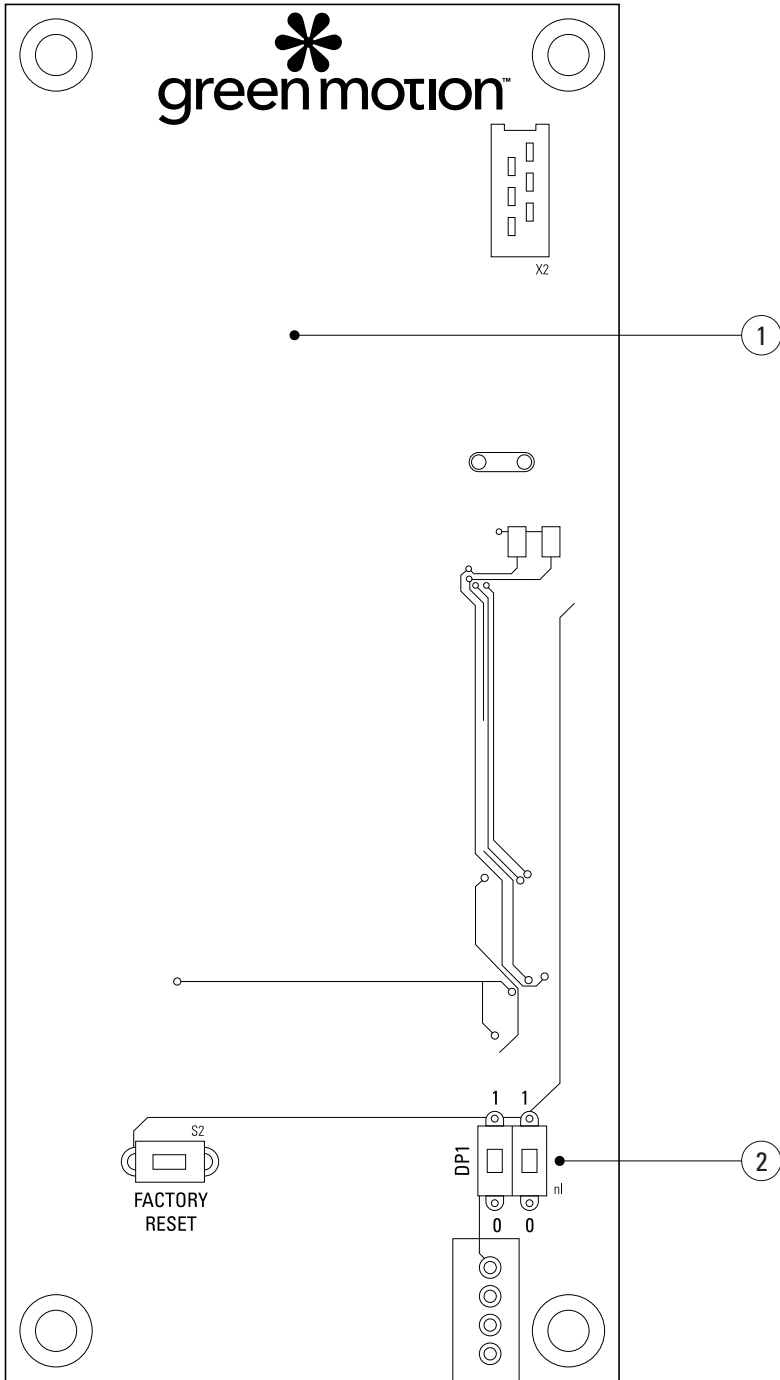
Figure 11. LED-Panel (PCB) located on the backside of the Green Motion Home EV charger front cover
