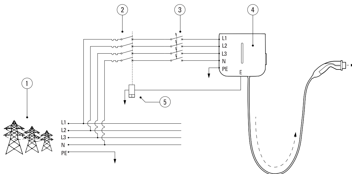
Figure 12. The Green Motion Home EV charger wiring diagram for EV-ready standards
