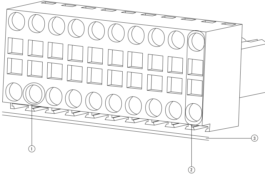
Figure 16. Proper alignment of the mating connector
