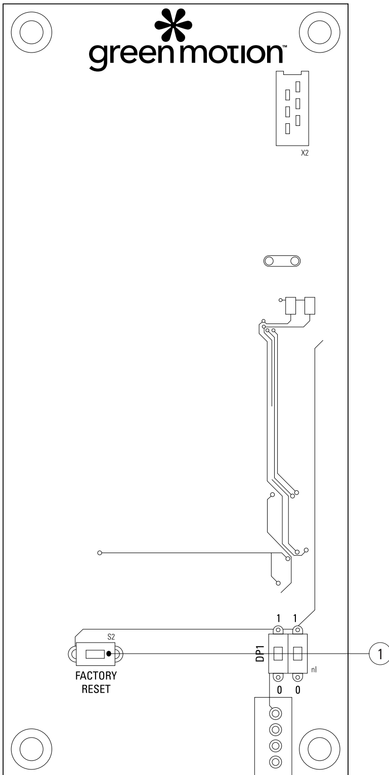
Figure 22. LED-Panel (PCB) located on the backside of the Green Motion Home EV charger front cover
