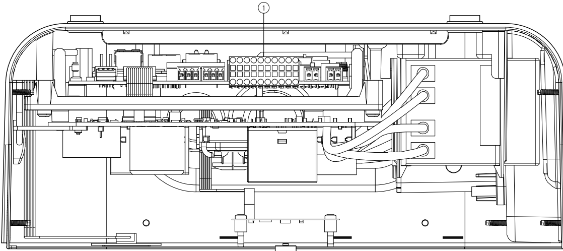
Figure 15. Top view showing the position of the J9 connector on the AC platform
