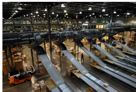
Material handling
