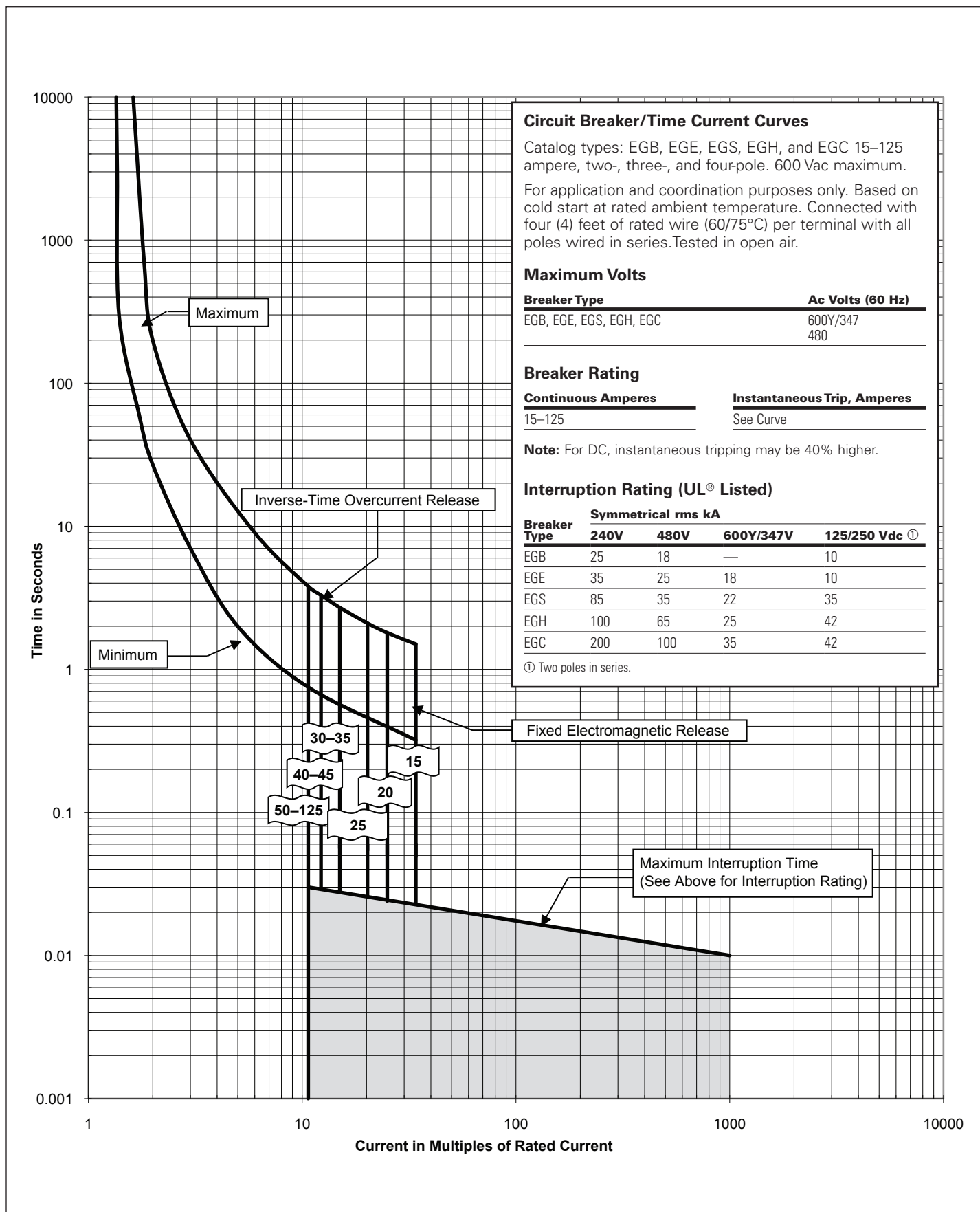
Figure 1. Type EGB, EGE, EGS, EGH, and EGC Two-, Three-, and Four-Pole Circuit Breakers
