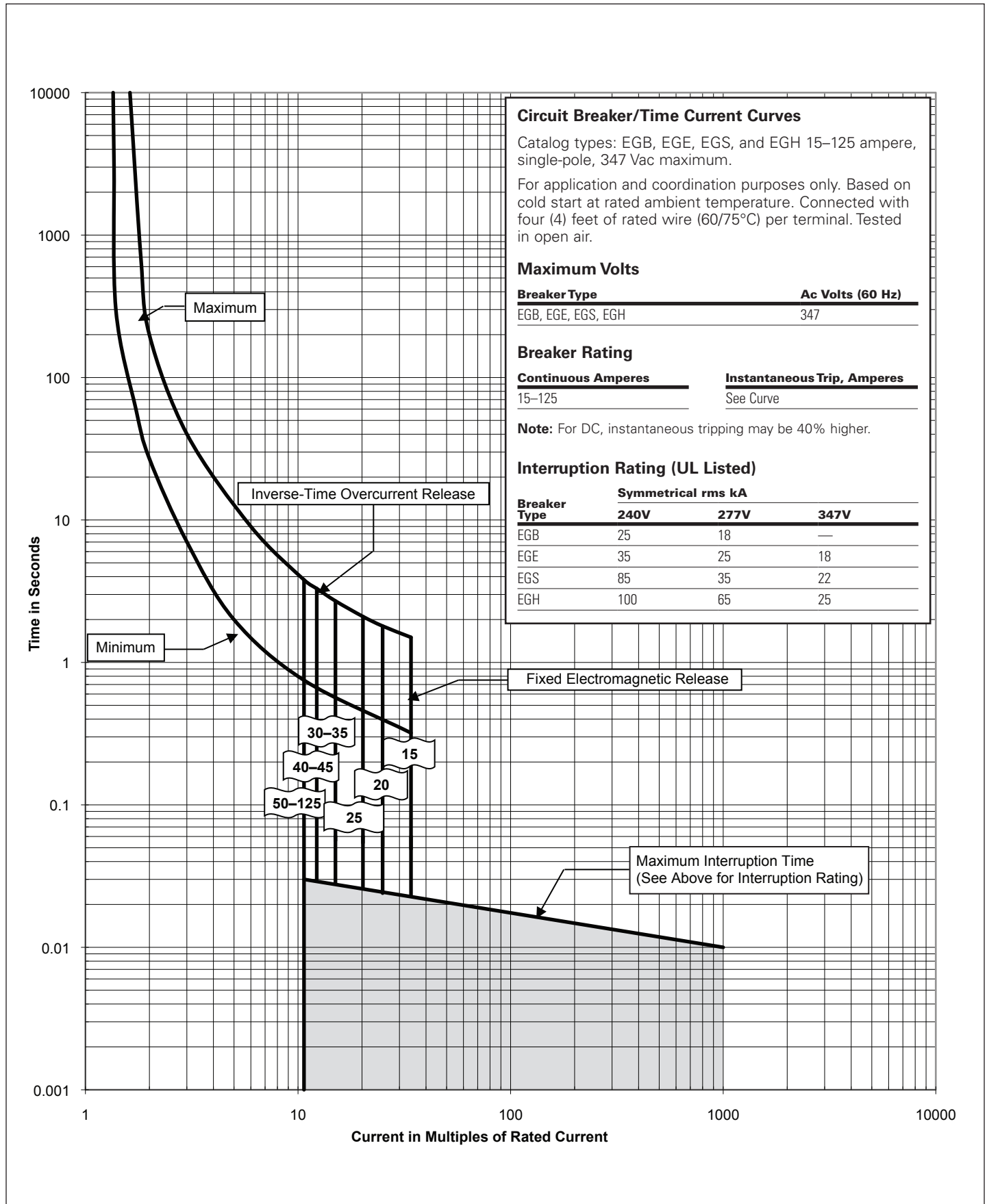
Figure 3. Type EGB, EGE, EGS, and EGH Single-Pole Circuit Breakers
