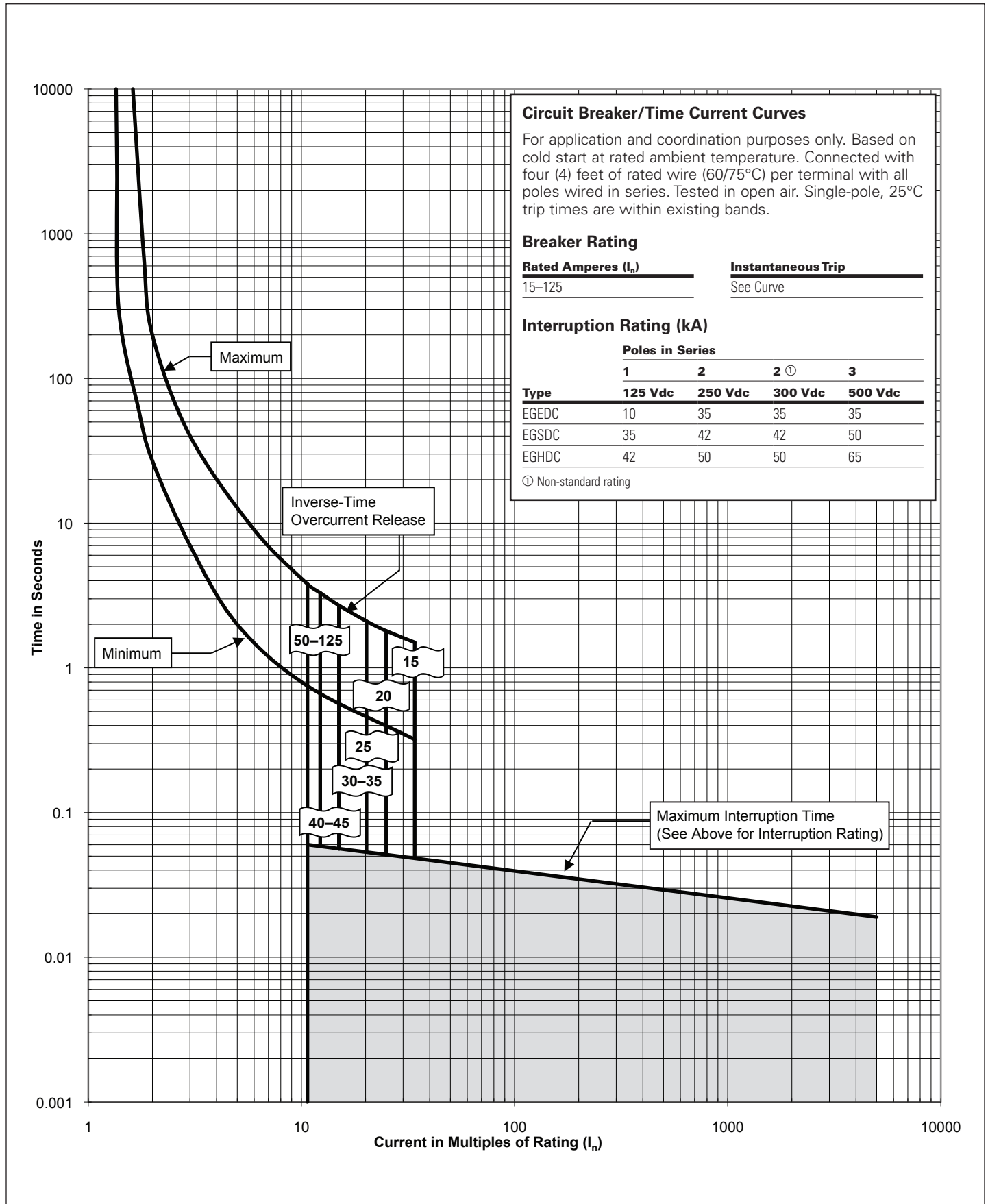
Figure 2. Type EGE, EGS, EGH, and EGK DC Circuit Breakers
