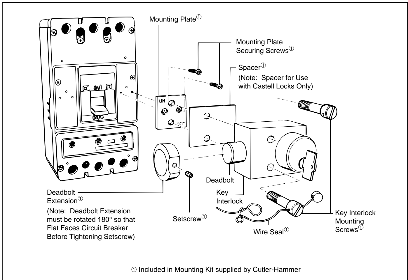
Figure 2-2 Key Interlock Installation (K-Frame Shown)
