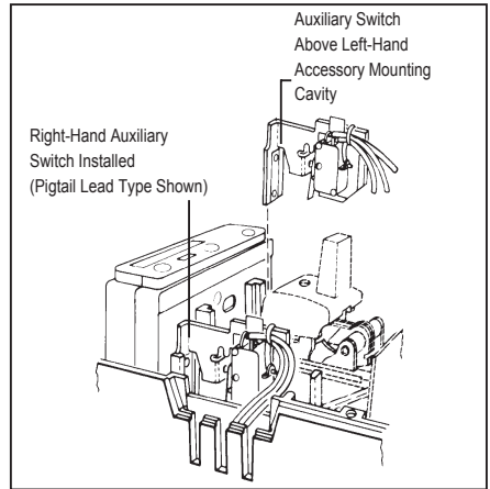
Fig. 2-3. Auxiliary Switch Installation Positions
