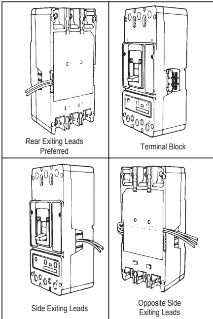
Fig. 2-2. Accessory Wiring Options
