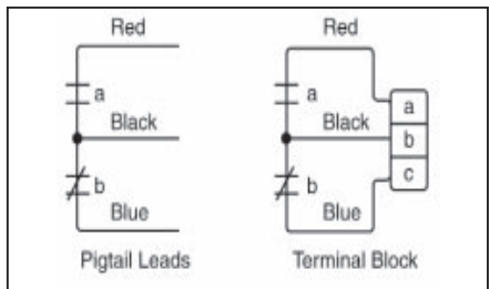
Fig. 2-6. Auxiliary Switch Connection Diagram
