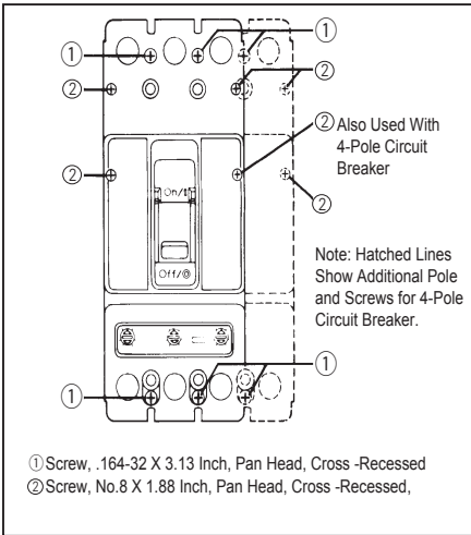
Fig. 2-4 Cover Screw Installation Positions
