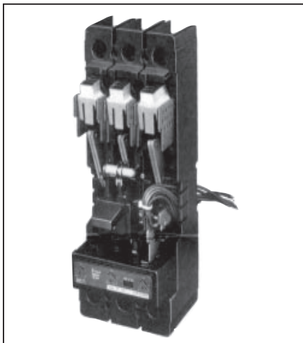
Fig. 1-1. Auxiliary Switch Installed in J-Frame Circuit Breaker
