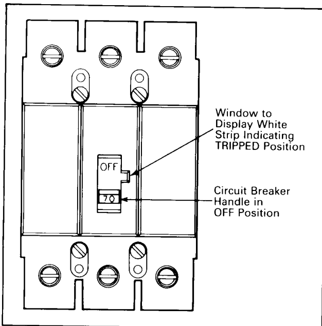
Fig. 3-1. Circuit Breaker Manual Controls
