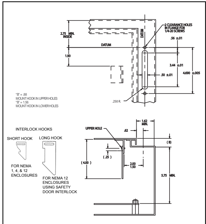
Fig. 1-8 Flange Drilling Plan for Handle and Interlock Blade Mounting Dimensions.
