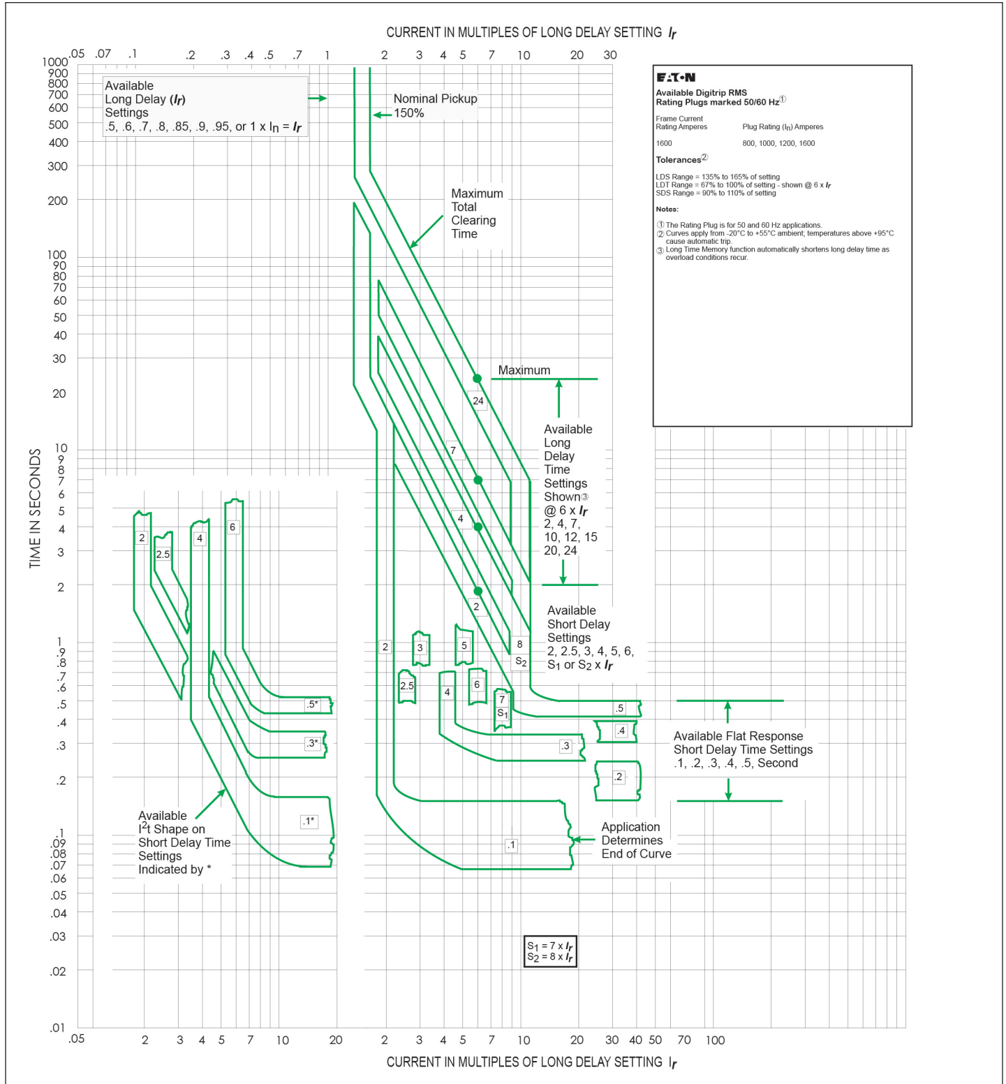
Navy AQB-A1603 Long Delay and Short Delay Time-Phase Current Characteristic Curve (LS):Curve Number: TC01218002E May 2017.
