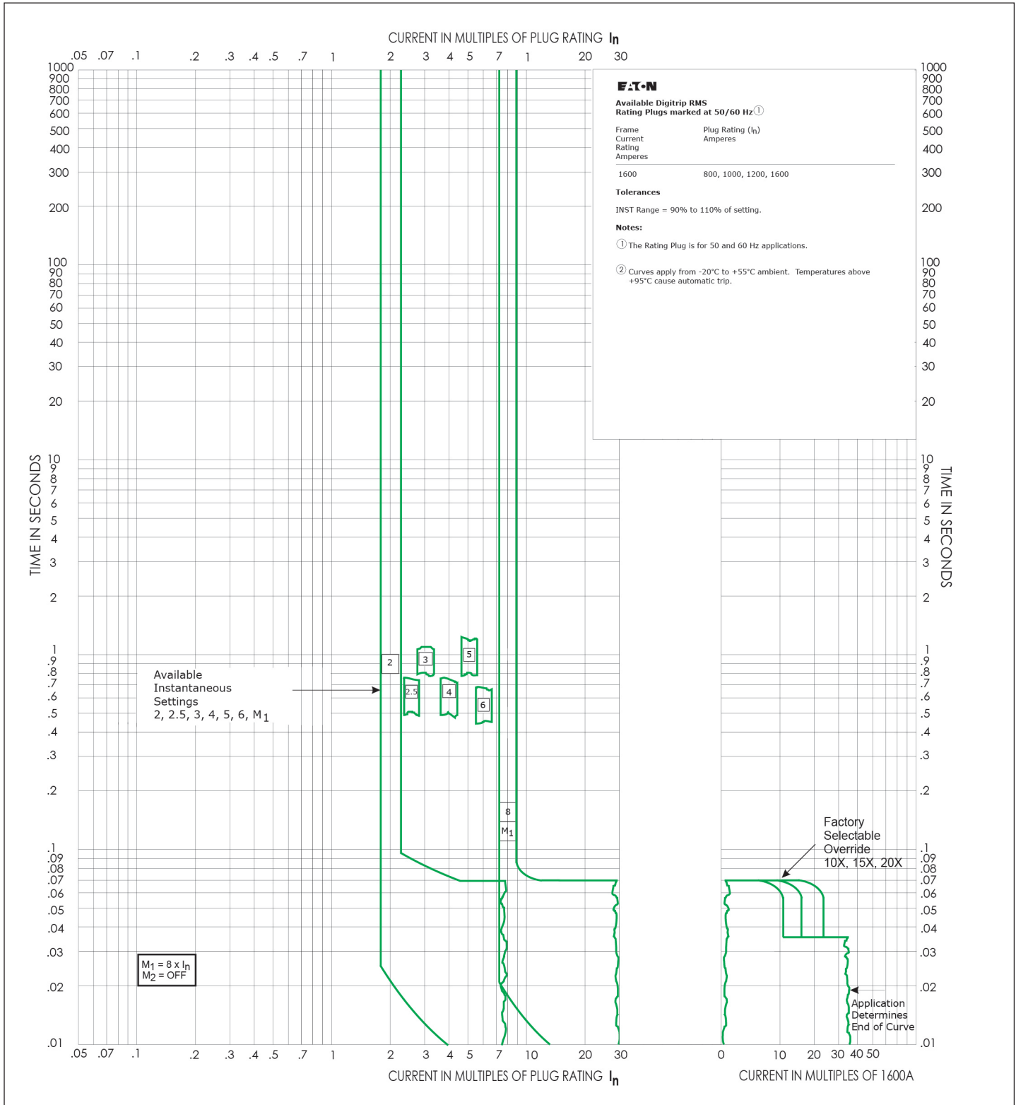
Navy AQB-A1603 Instantaneous Time-Phase Current Characteristic Curve (I):
