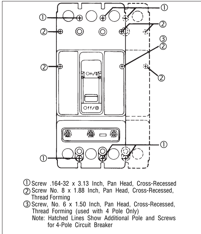
Figure 7. Cover Screw Installation Positions.
