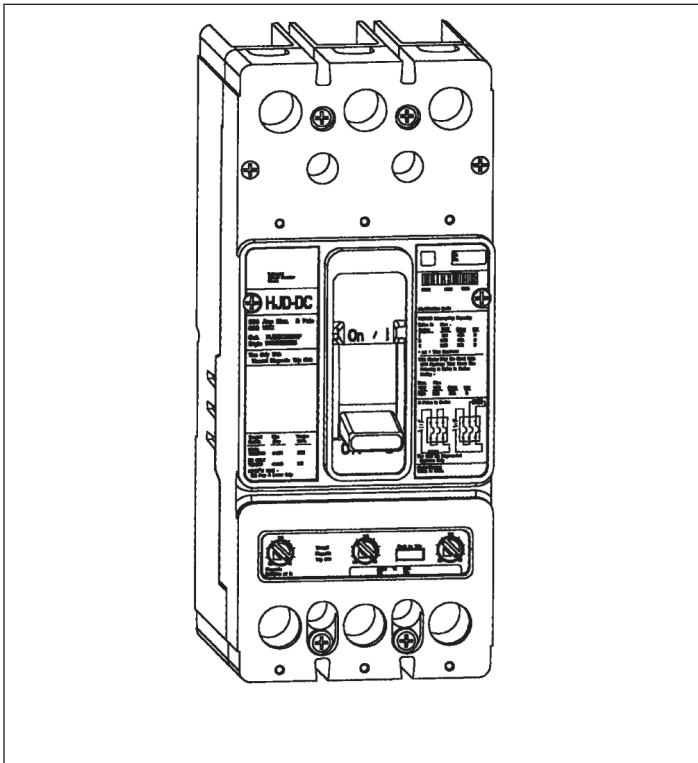
Figure 1. Type HJDDC Series C DC Circuit Breaker with JT Trip Unit Installed.
