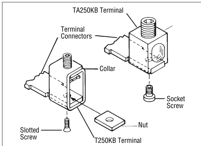
Figure 8. Terminal Installation.
