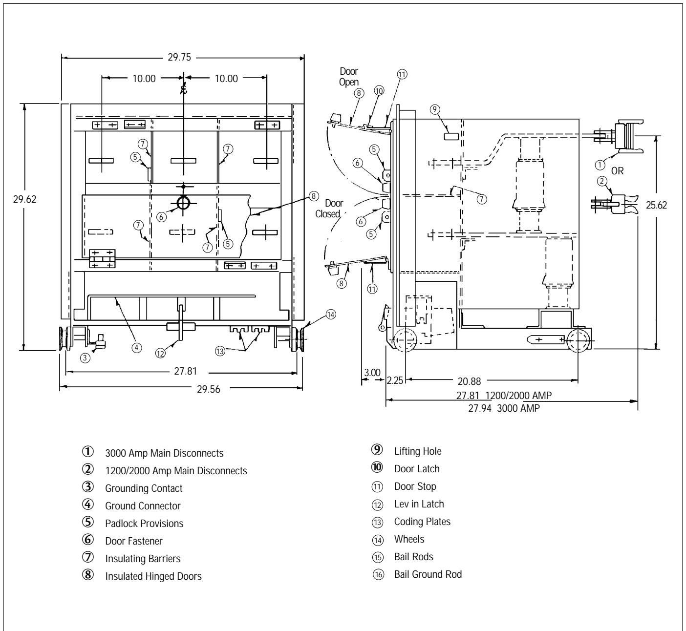
Figure 4 Standard Device (Upper)
