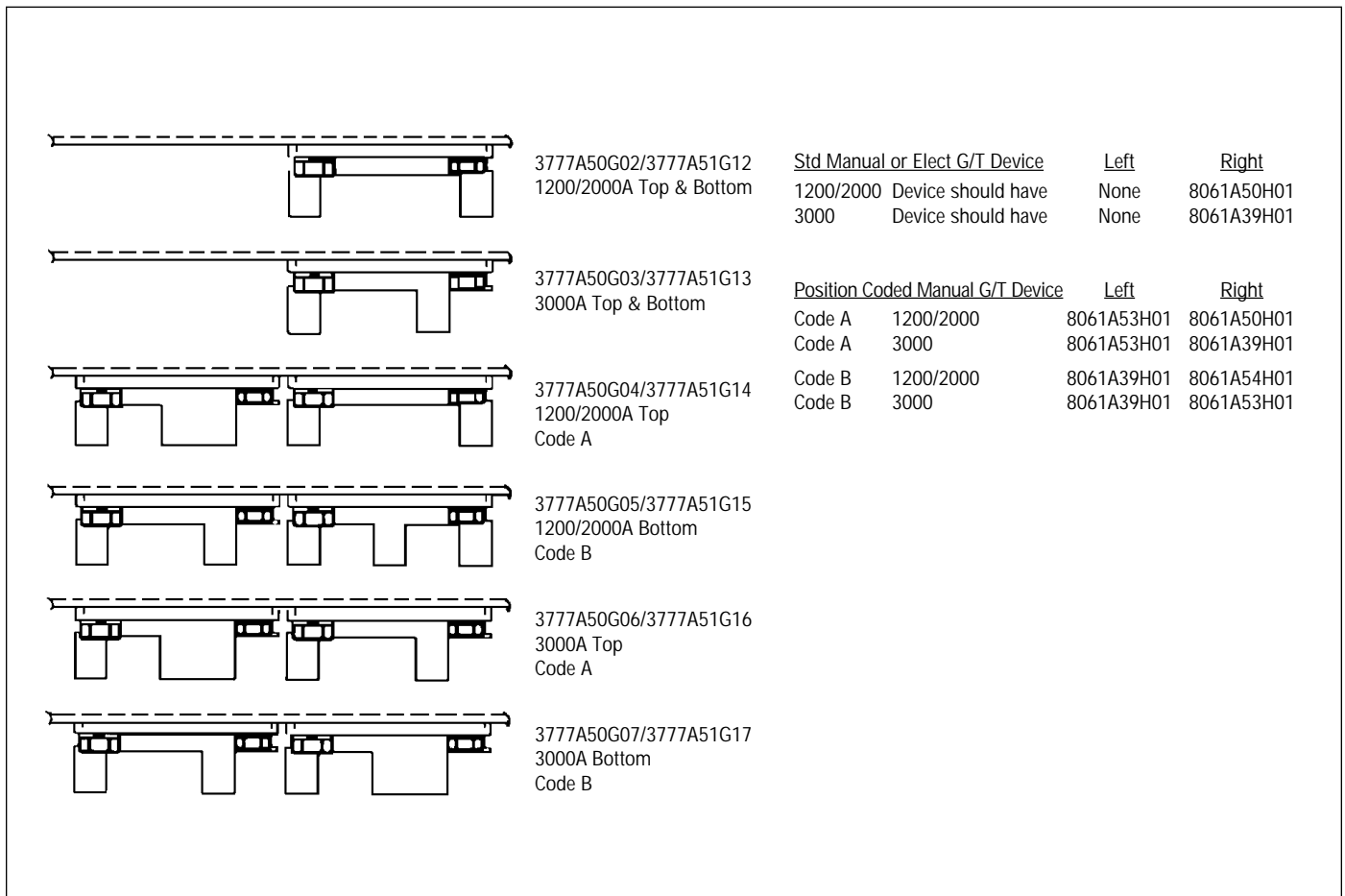
Figure 8 Code Plate Legend
