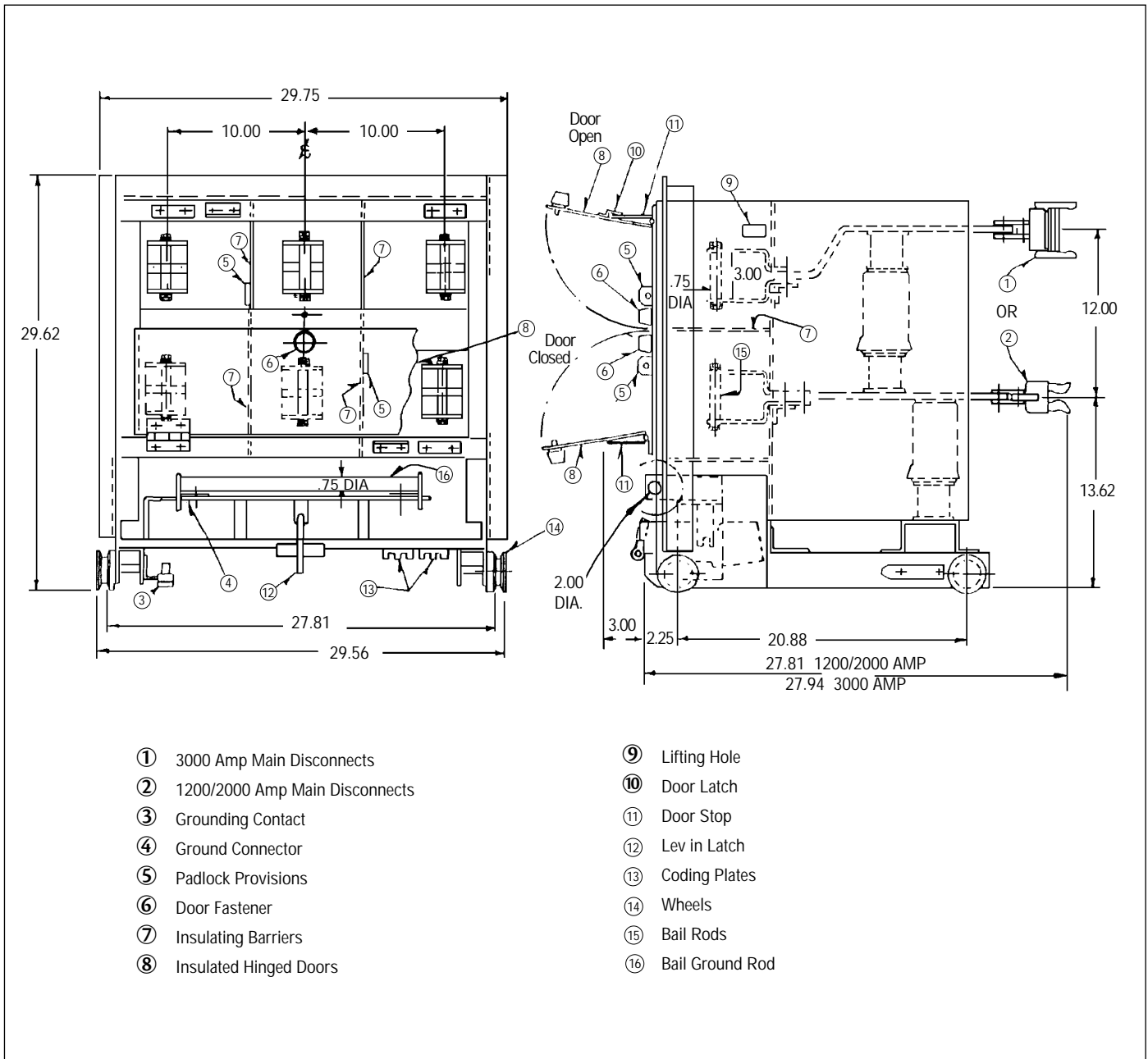
Figure 3 Device With Bails
