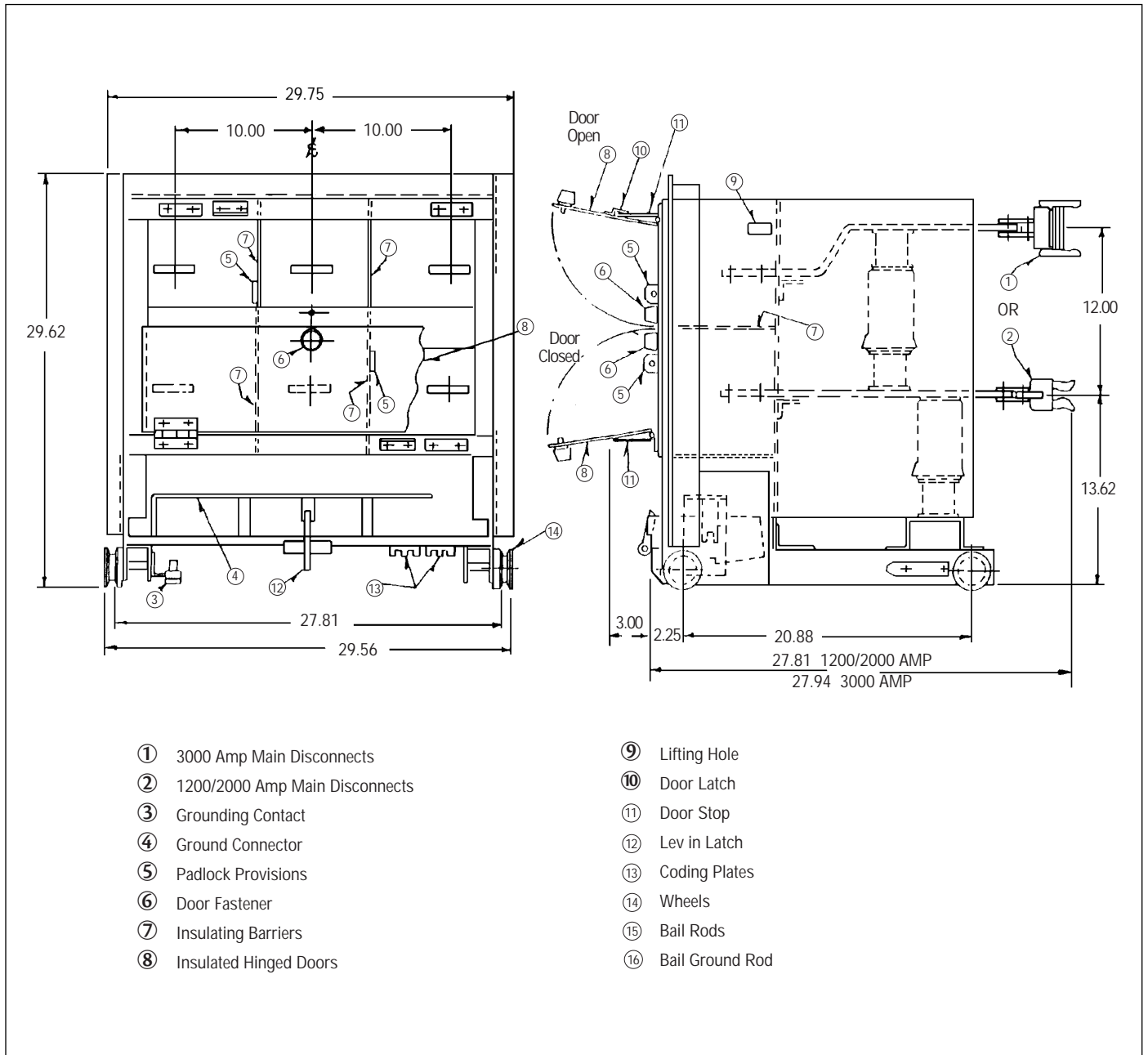
Figure 2 Standard Device
