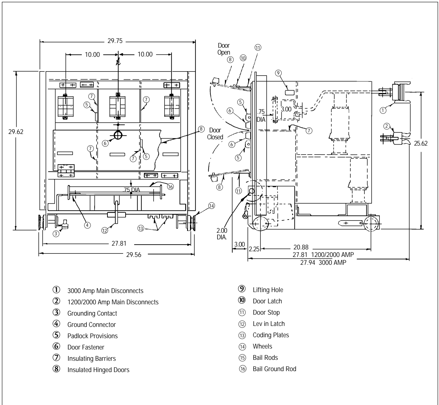
Figure 6 Device With Bails (Upper)
