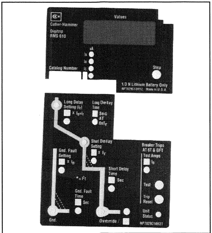
Fig. 3.5 Digitrip RMS 610 Type LSG
