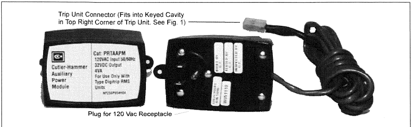
Fig. 7 Auxiliary Power Module
