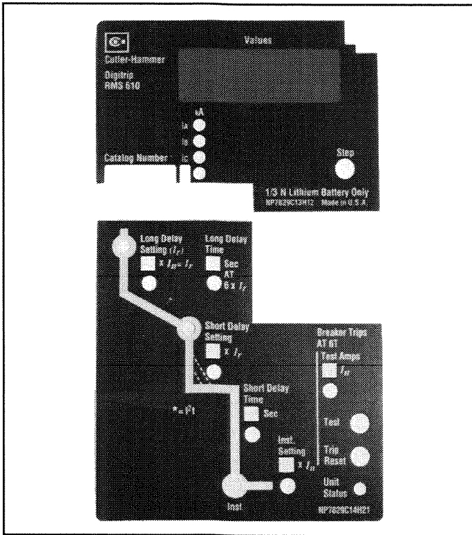
Fig. 3.3 Digitrip RMS 610 Type LSI
