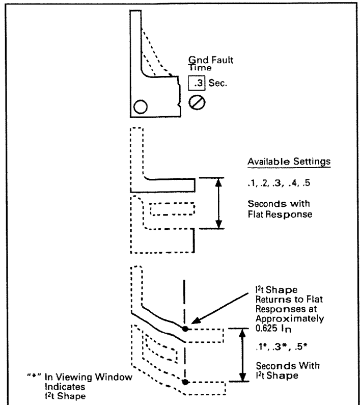
Fig. 8.7 Ground Fault Time Delay Setting
