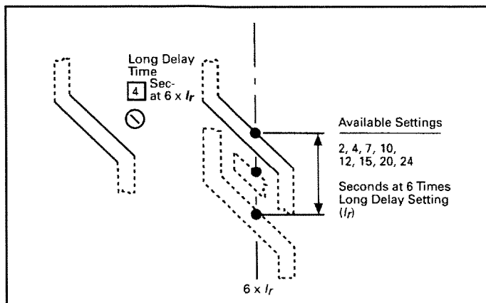
Fig. 8.2 Long Delay Time Settings
