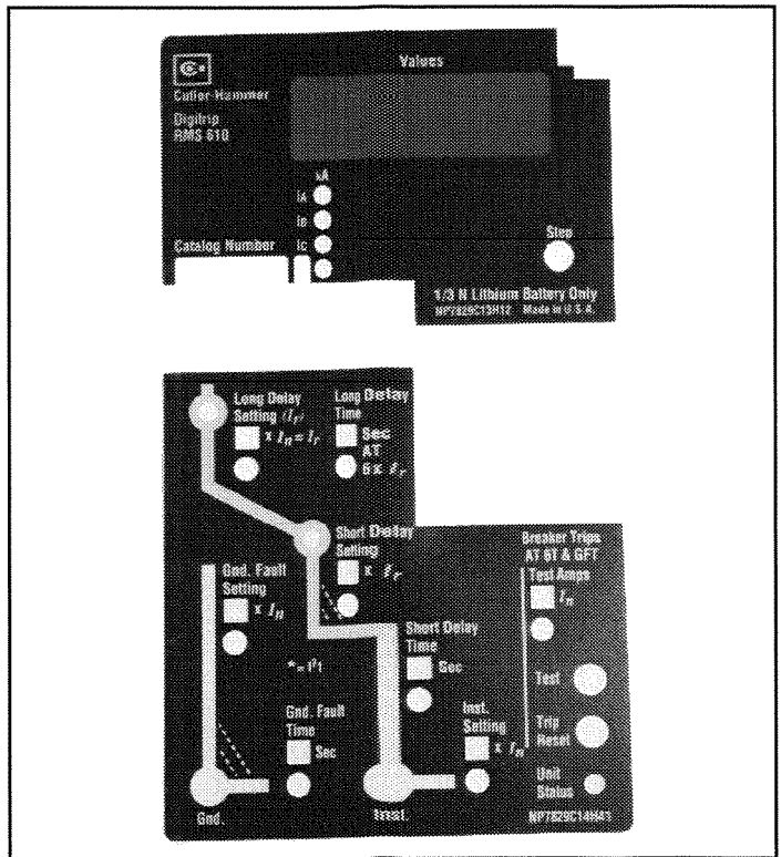
Fig. 3.6 Digitrip RMS 610 Type LSIG
