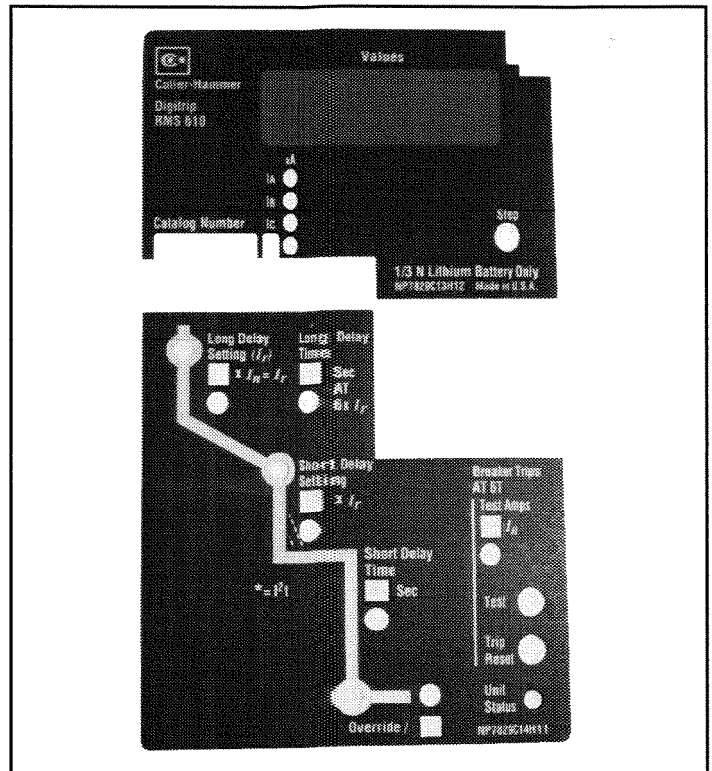
Fig. 3.2 Digitrip RMS 610 Type LS
