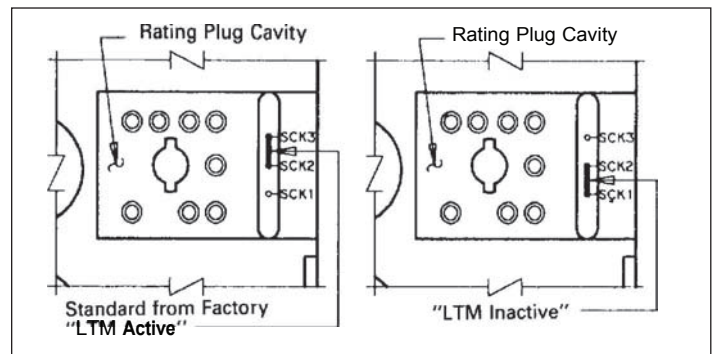
Figure 13. Long Time Memory "LTM" Jumper.
