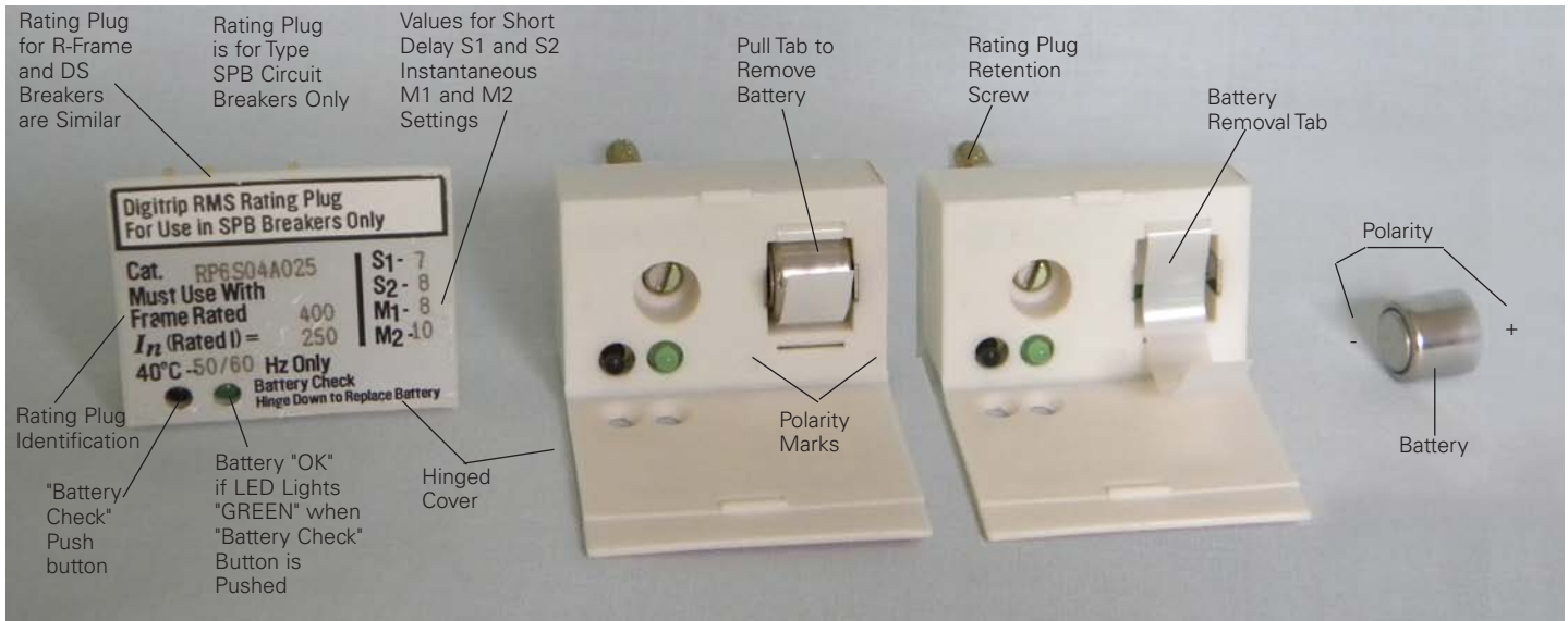
Figure 9. Rating Plug.
