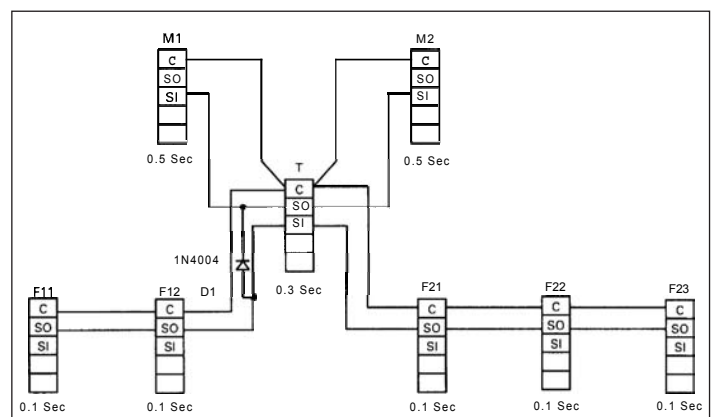
Figure A.2 Typical Zone Interlocking Connections with Two Main Breakers (M1, M2) and a Tie Breaker (T) (Short Delay Protection).
