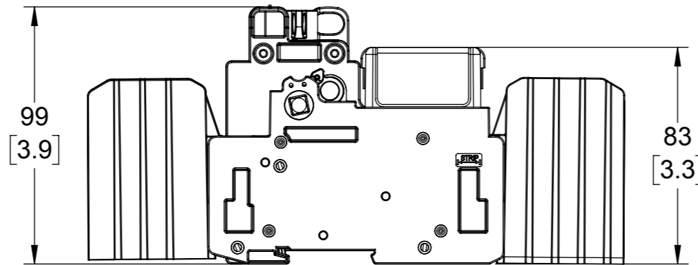
30A CUBE Fuse Installed
