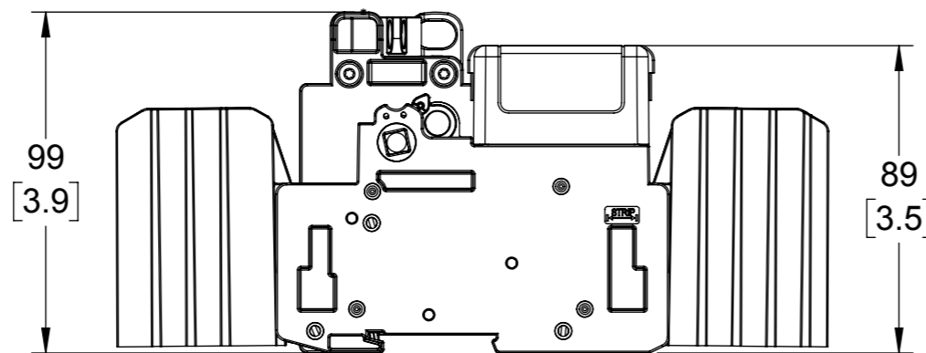
60A CUBE Fuse Installed
