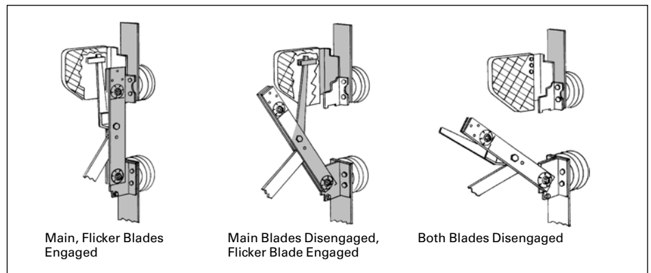
Figure 8.3-1. Switch Operation
