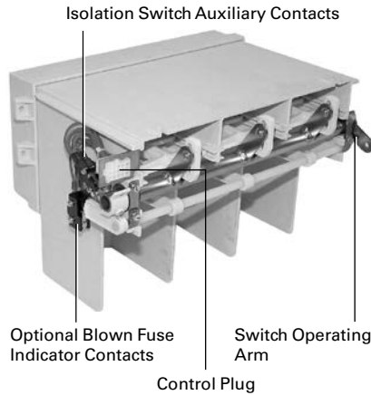
JMT-400/800 A Isolation Switch Front View
