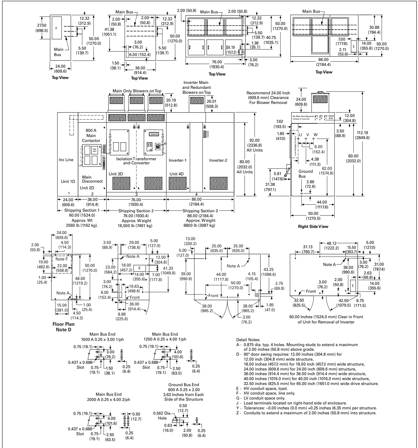
Figure 10.4-8. SC9000 EP VFD Frame D (Parallel Inverters) Maximum Dimensions and Incoming Line Layouts—Dimensions in Inches (mm)
