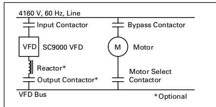
Figure 10.4-14. Closed Transition Synchronous Transfer Elements
