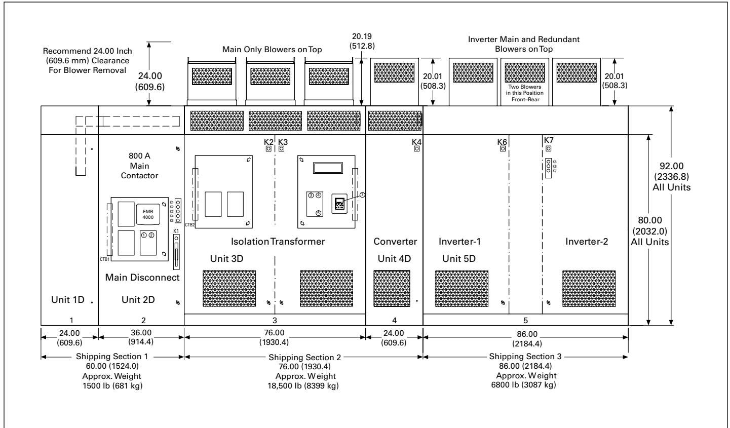
Figure 10.4-9. SC9000 EP Frame E—Dimensions in Inches (mm)
