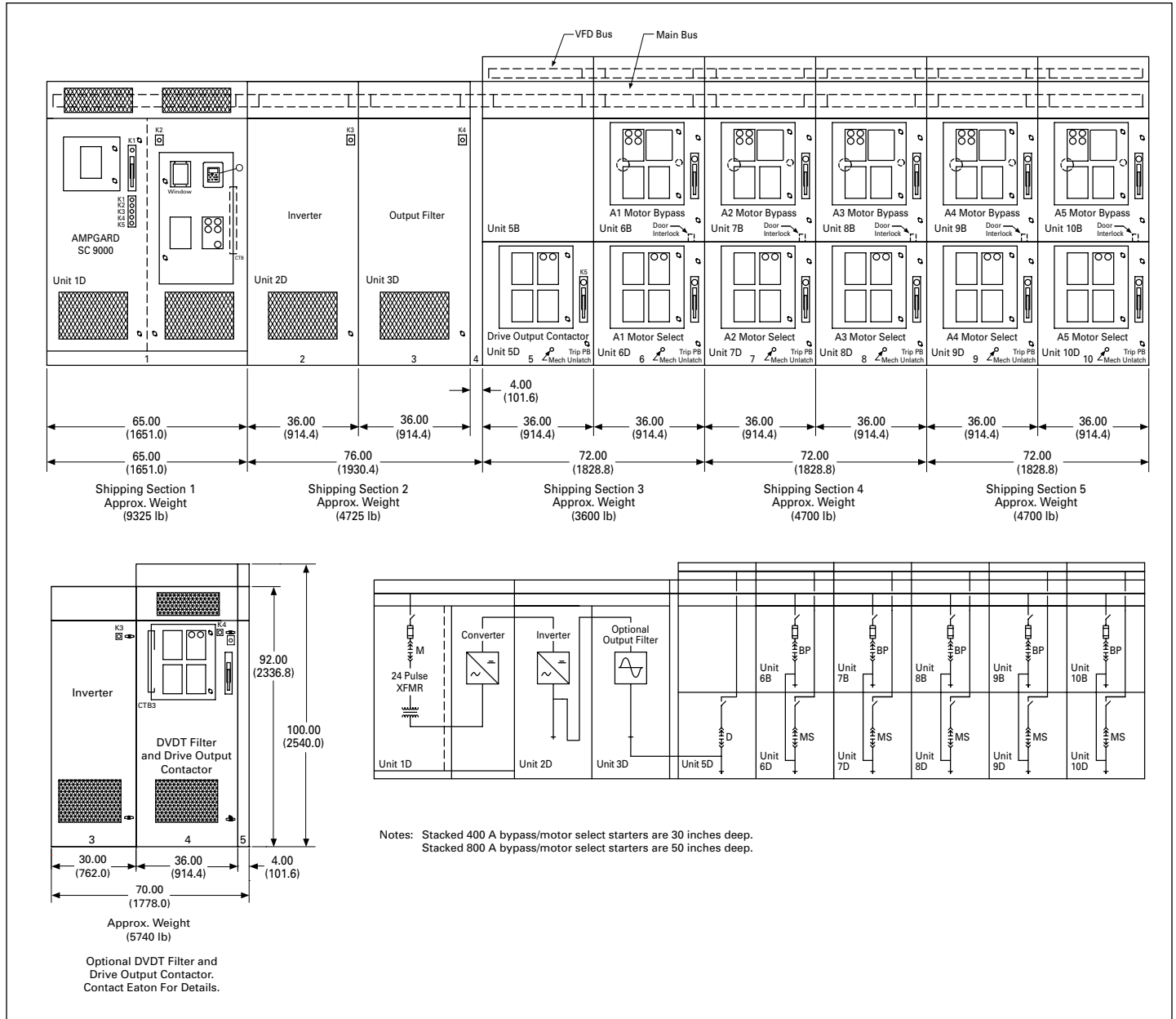
Figure 10.4-13. SC9000 EP Synchronous Transfer System with Five MV Starters (For Reference Only)
