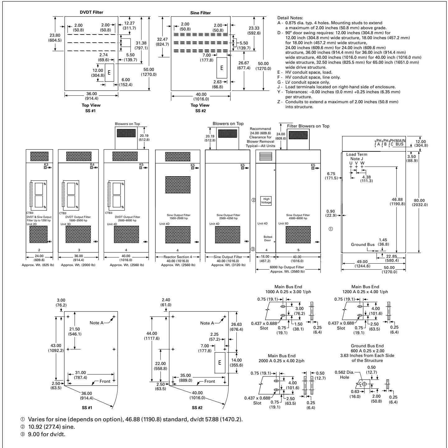
Figure 10.4-12. SC9000 EP VFD Output Filter Maximum Dimensions and Incoming Line Layouts—Dimensions in Inches (mm)
