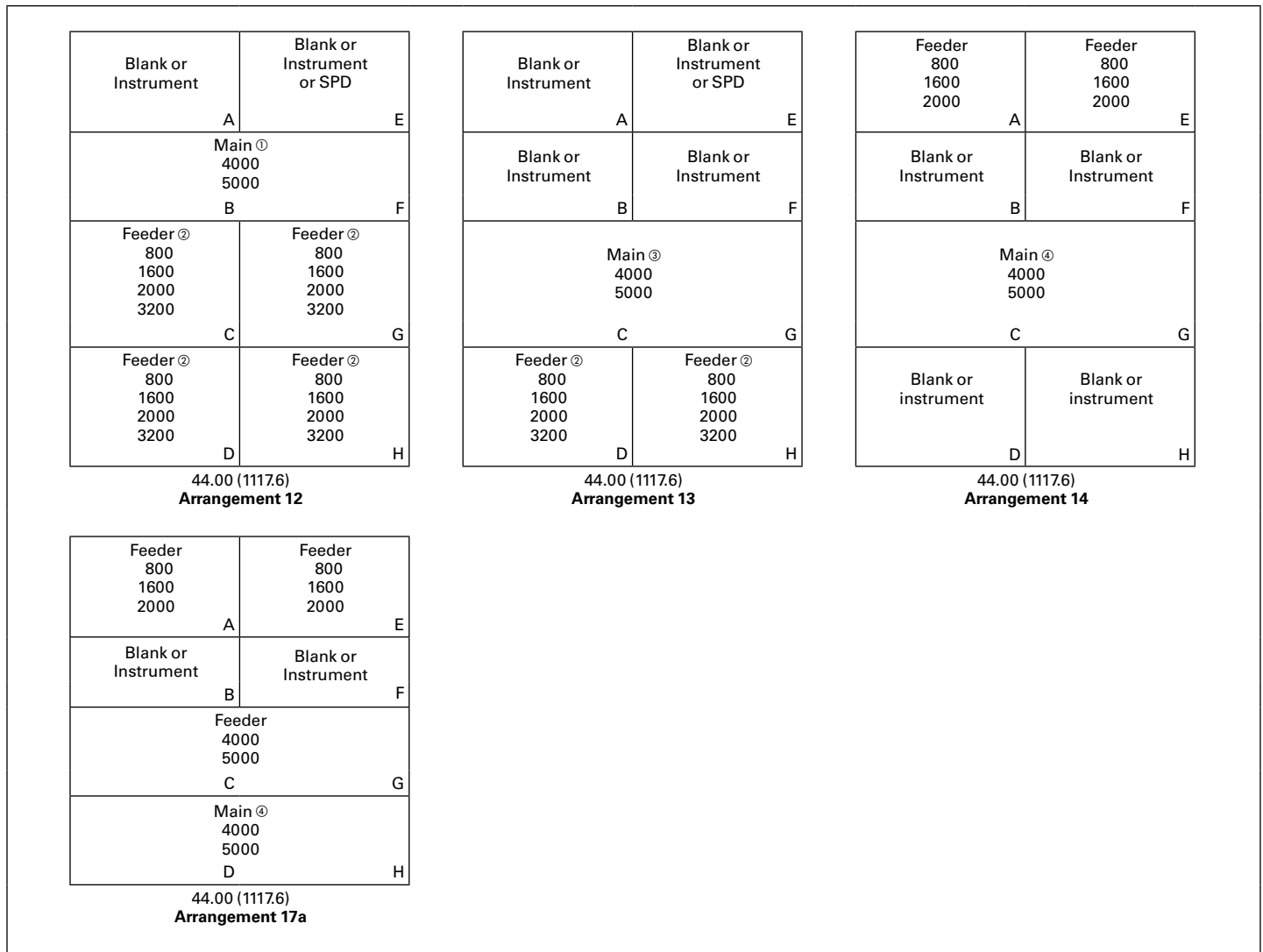
Figure 20.1-6. Typical Structure and Breaker Arrangements (Continued)—Magnum DS Mains, 4000 A and 5000 A
