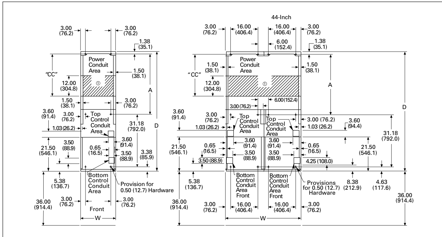
Figure 20.1-8. Floor Plans and Available Conduit Space—18.00, 22.00, 30.00, 44.00-Inch (457.2, 558.8, 762.0, 1117.6 mm) Wide Rear-Access Structures—Dimensions in Inches (mm)
