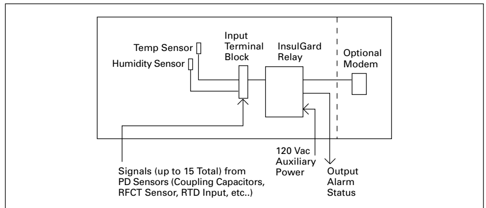
Figure 6.1-8. InsulGard Relay System
