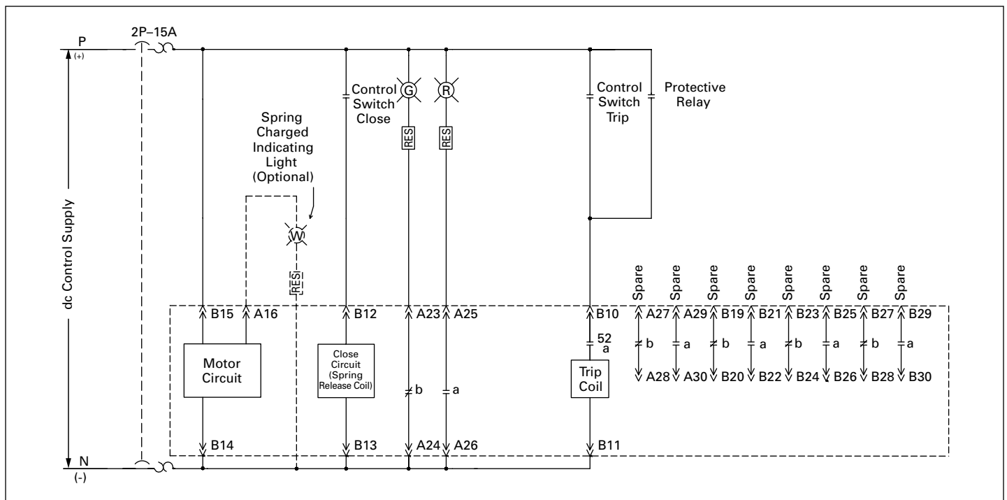
Figure 6.1-19. Typical dc Control Circuit—VCP-T Breaker
