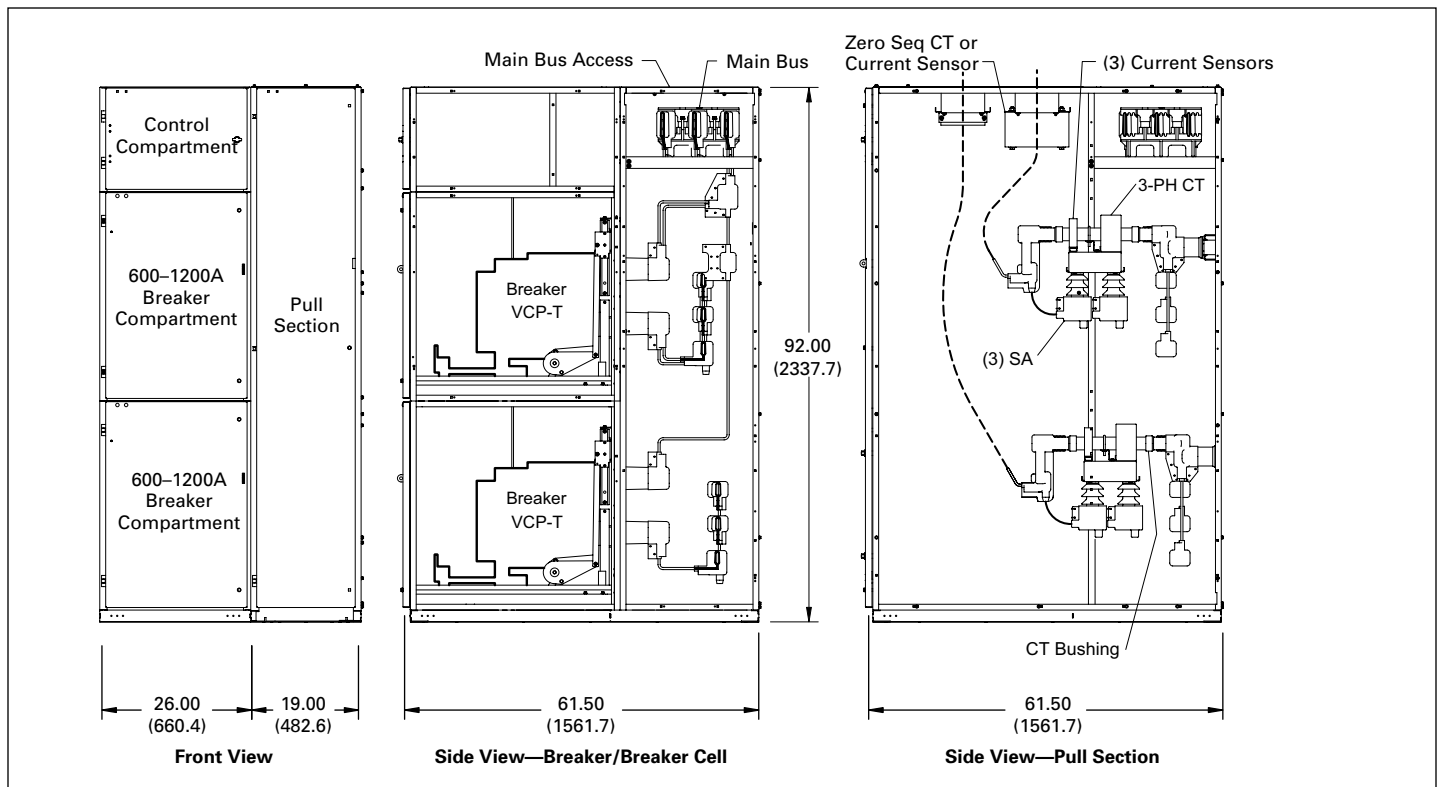
Figure 6.1-14. Typical Breaker/Breaker Unit and Pull Section, Cables Out the Top
