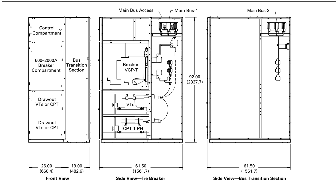
Figure 6.1-15. Typical Bus Tie Breaker Unit and Bus Transition Section
