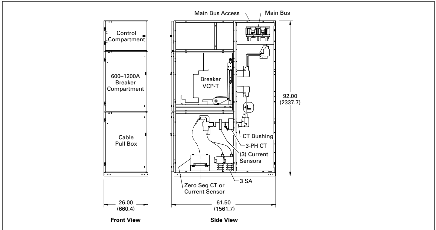
Figure 6.1-11. Typical 1-High Breaker Unit, Cables Out the Bottom
