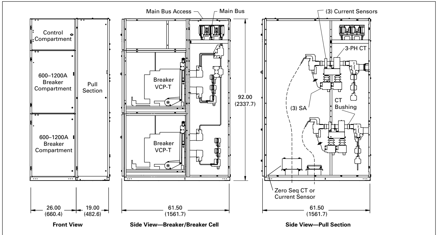
Figure 6.1-13. Typical Breaker/Breaker Unit and Pull Section, Cables Out the Bottom
