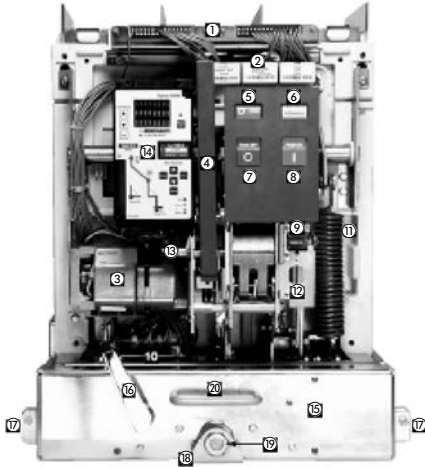
VCP-T Breaker
