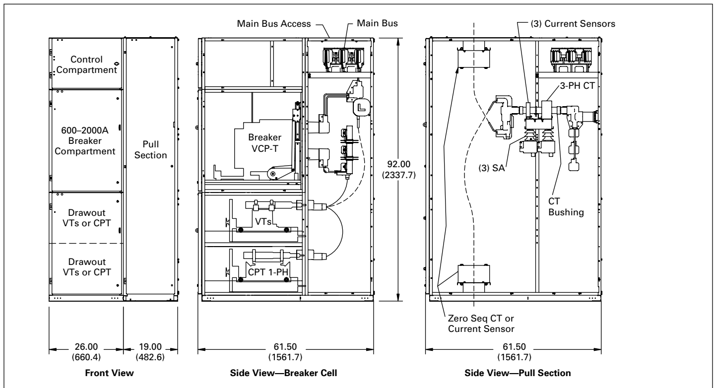
Figure 6.1-12. Typical Breaker/Auxiliary Unit and Pull Section, Cables Out Top or Bottom
