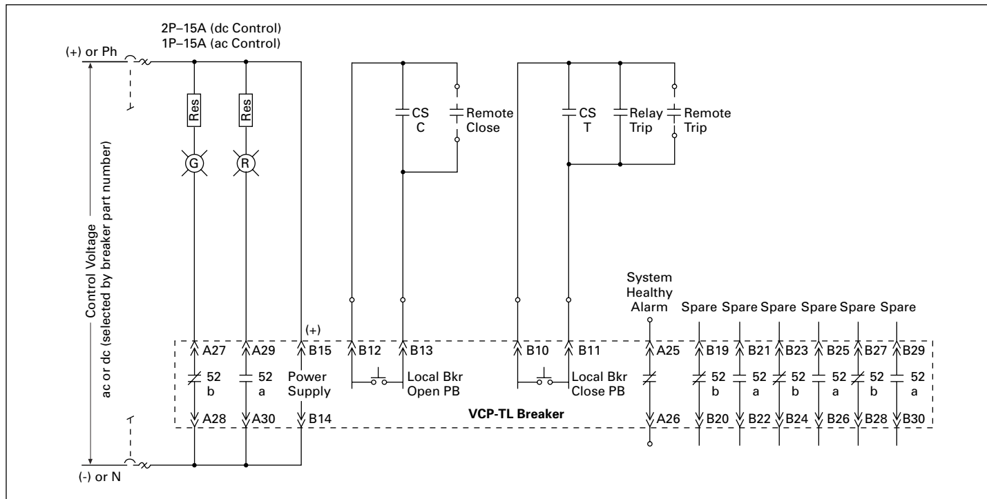
Figure 6.1-20. VCP-TL Circuit Breaker—Typical Control Circuit
