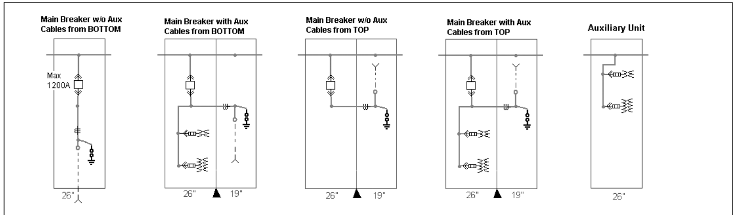
Figure 6.1-10. MEF Switchgear—Available Configurations
