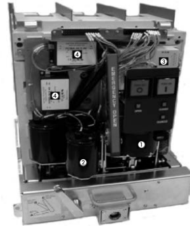
VCP-TL Breaker
