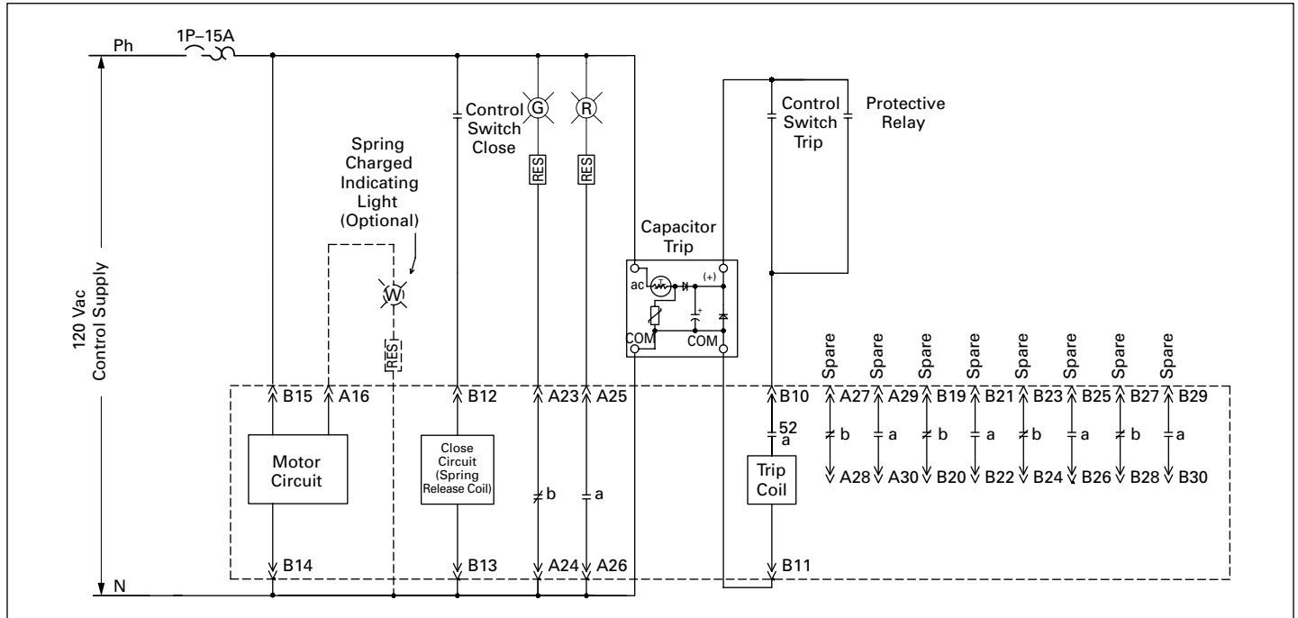
Figure 6.1-18. Typical ac Control Circuit—VCP-T Breaker
