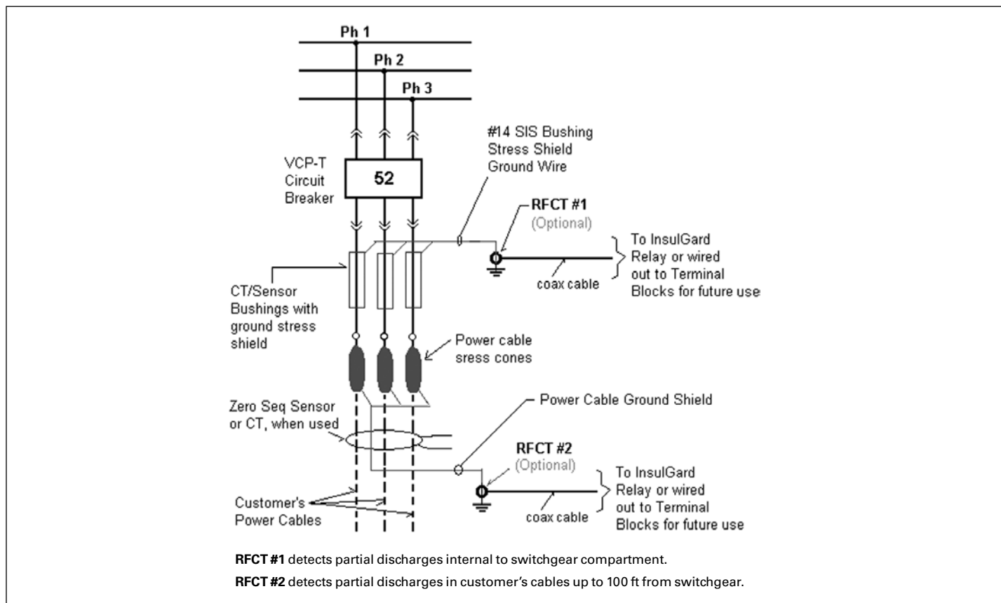
Figure 6.1-9. Typical Partial Discharge Sensor Connections in MEF Switchgear (5–15 kV)
