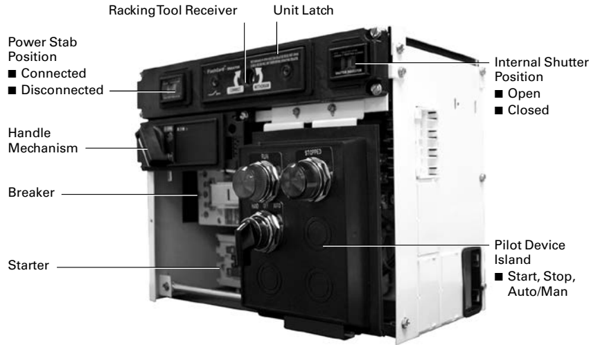
Freedom FlashGard FVNR Starter
