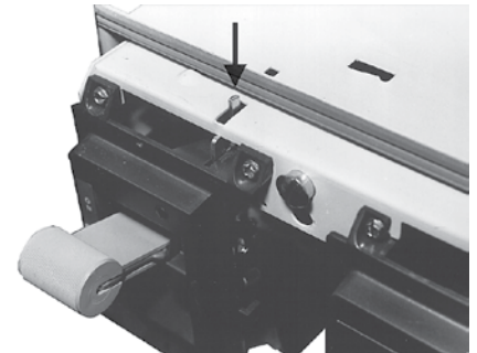
Unit Insertion Interlock
