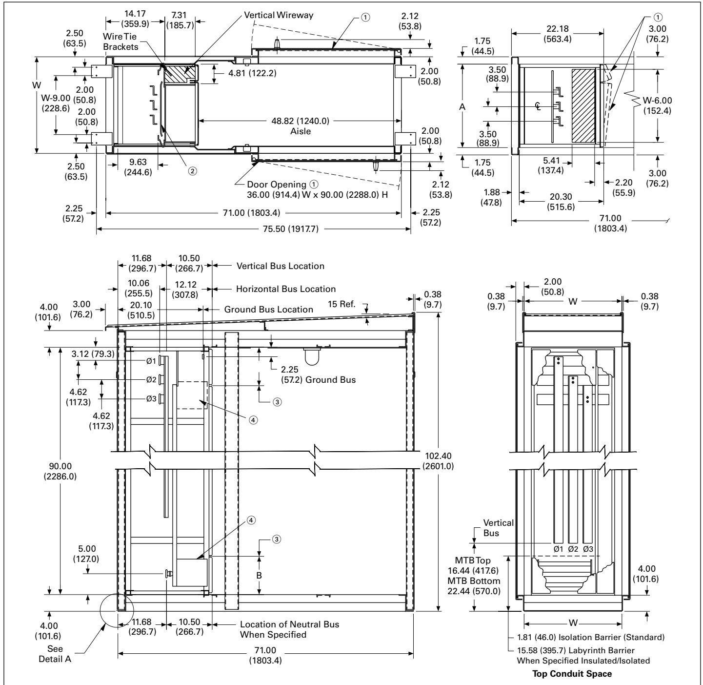
Figure 29.1-14. Freedom and Freedom FlashGard NEMA 3R Walk-In Aisle Structures—Dimensions in Inches (mm)
