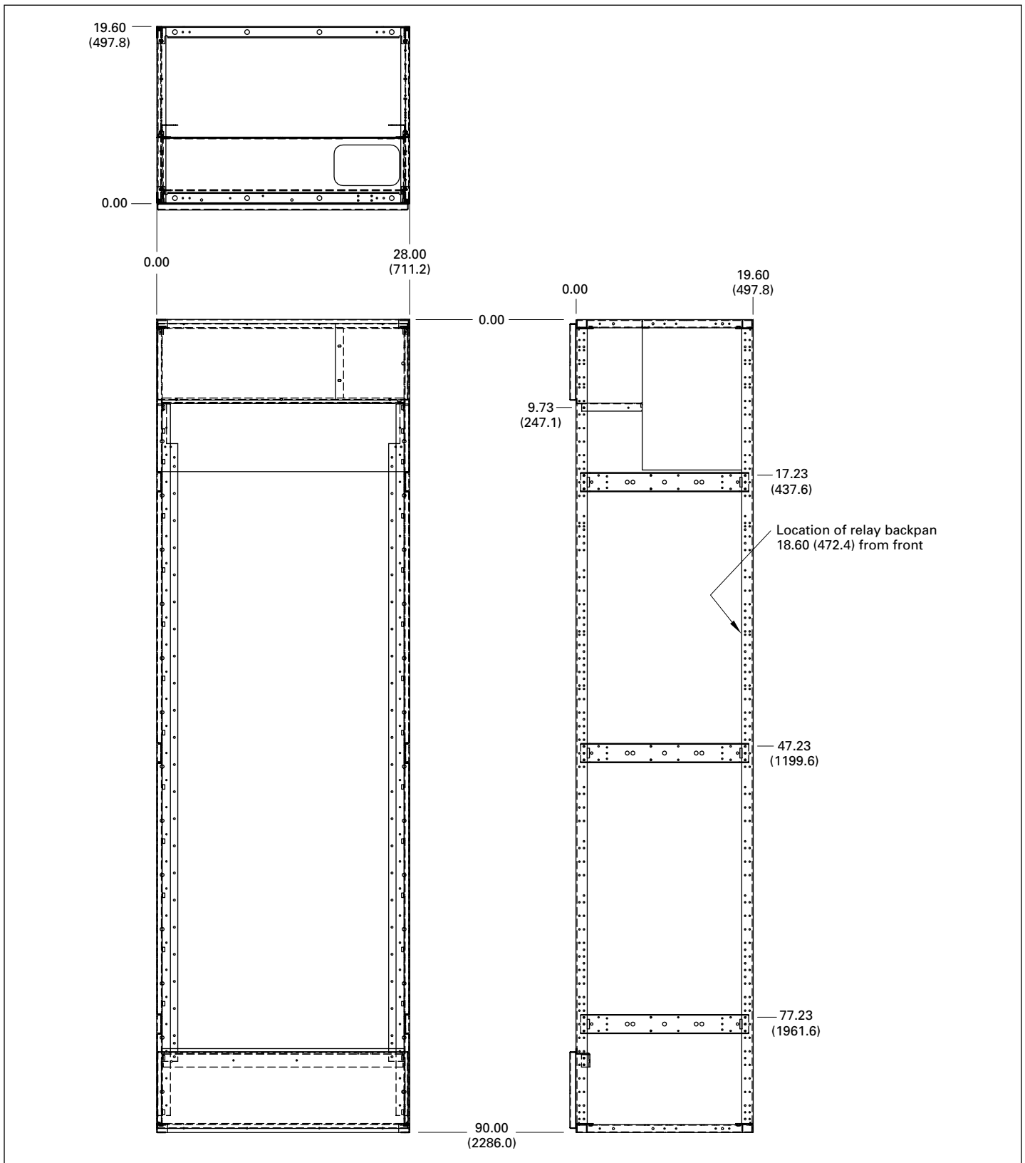
Figure 29.1-6. Relay Structure (28.00 inches [711.2 mm] wide and 20.00 inches [508.0 mm] deep shown)
