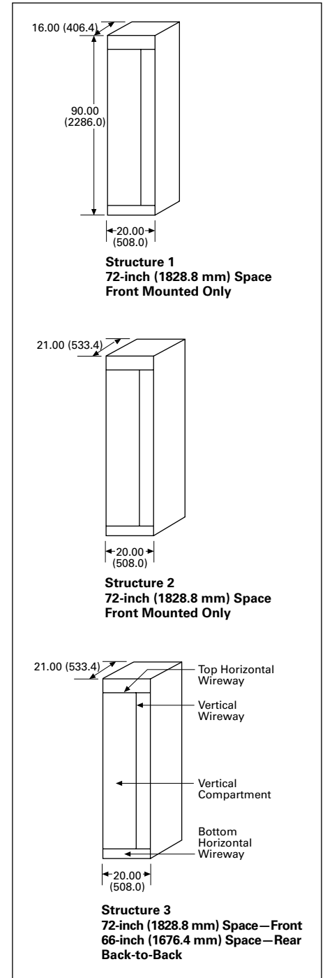
Figure 29.1-1. Structure—Dimensions in Inches (mm)
