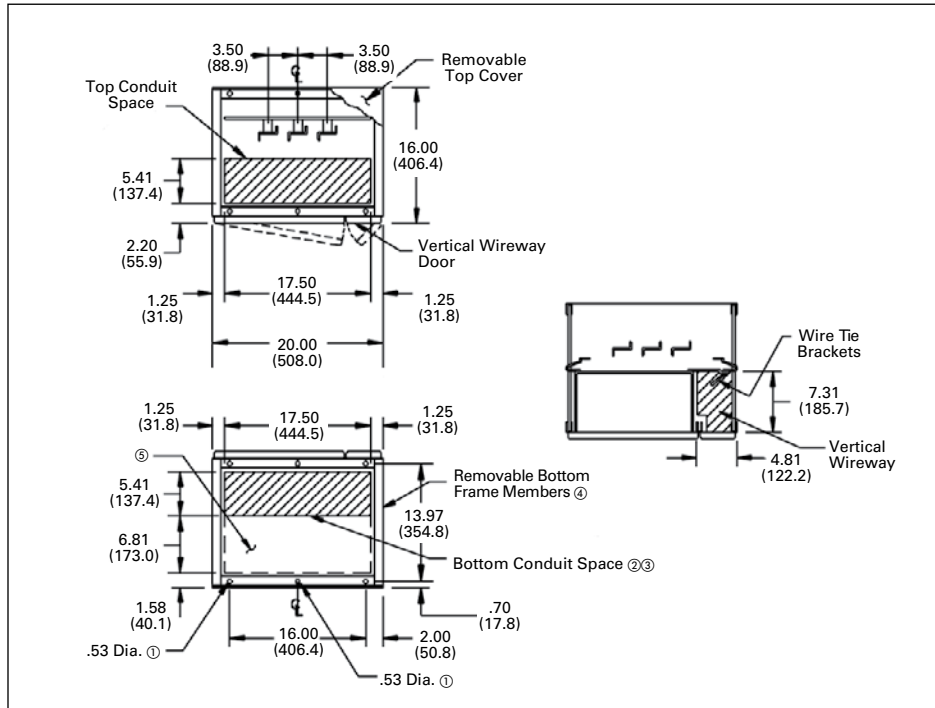
Figure 29.1-7. 20.00 Inches (508.0 mm) Wide, 16.00 Inches (406.4 mm)—Deep-Front Mounted Only (FMO)—Dimensions in Inches (mm)
