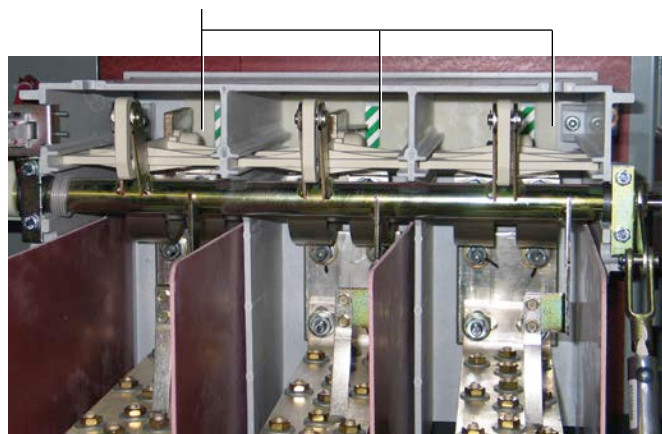
View of Isolation Switch Through Viewing Window
