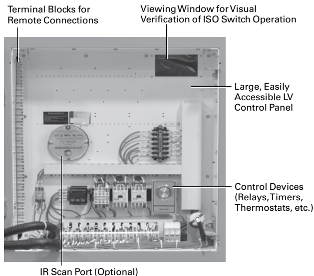
Ampgard Starter—Low-Voltage Compartment
