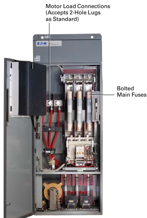
Ampgard 300 A Starter—Medium-Voltage Door Open
