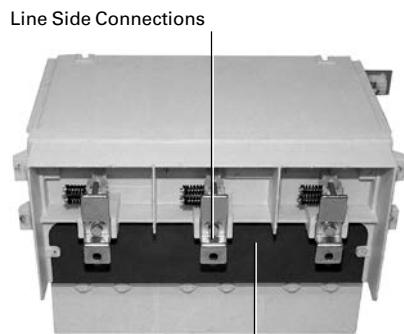
JMT-400/800 A Isolation Switch Rear View
