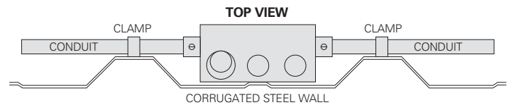
Elevated side knockouts eliminate the need for conduit bends
