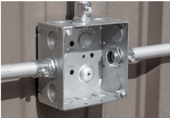
Elevated side knockouts eliminate the need for conduit bends
