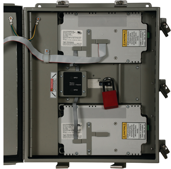
SPD MAX with safety barriers and optional circuit breaker locked out
