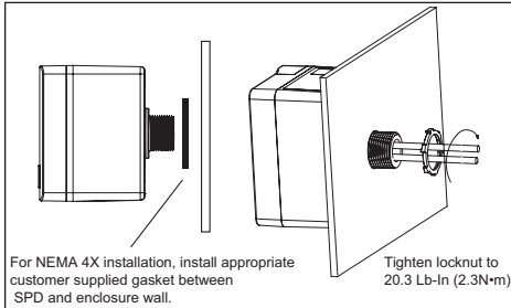
Figure 2-1. Panel Installation
