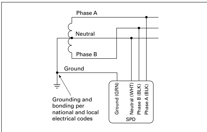
Figure 7. Split-phase (1S101)
