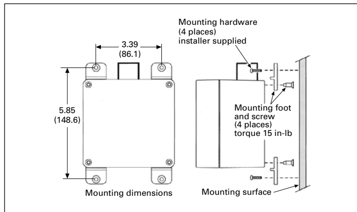
Figure 4. Wall mounting using external mounting feet
