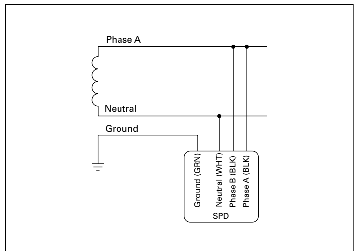
Figure 11. Single-phase 120 V (1S101)
