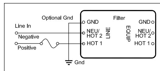
Figure 6. Parallel DC Application
