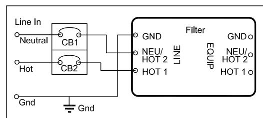
Figure 5. Split Phase Parallel AC Application (shown with Neutral utilized as NEU/HOT 2)
