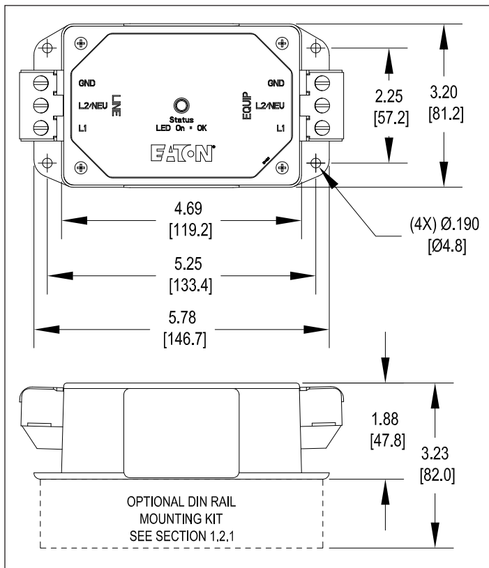
Figure 7. Product Dimensions
