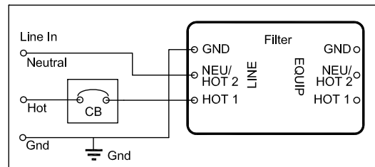
Figure 4. Single Phase Parallel AC Application
