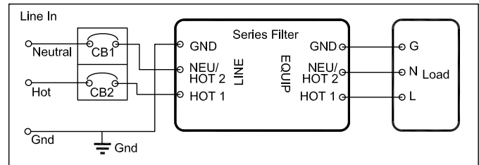
Figure 2. Split Phase Series AC Application (shown with Neutral utilized as NEU/HOT 2)
