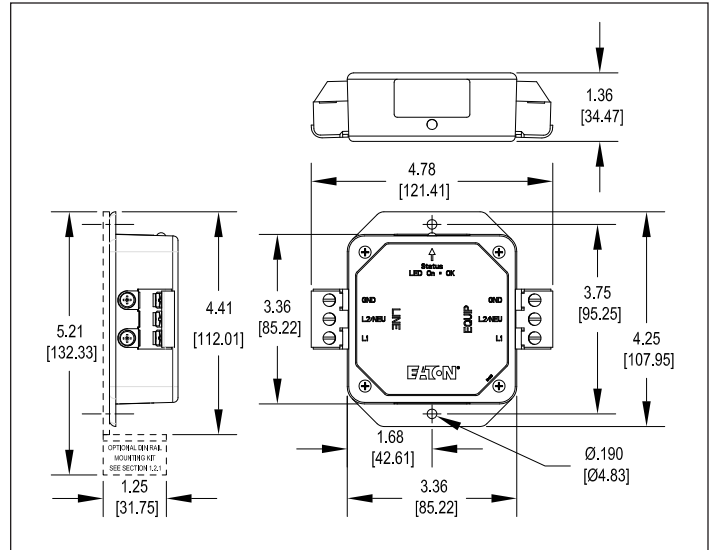
Figure 7. Product Dimensions
