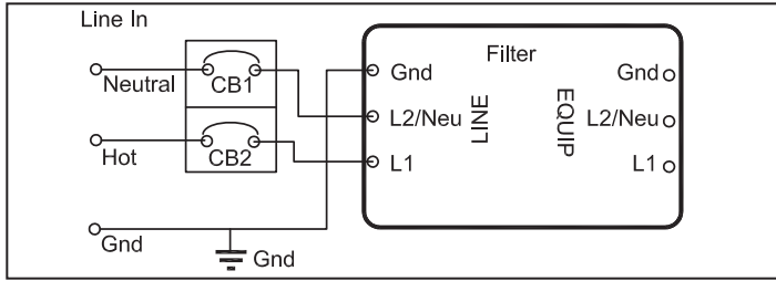
Figure 5. Split Phase Parallel AC Application (Shown with Neutral Utilized as L2/NEU)
