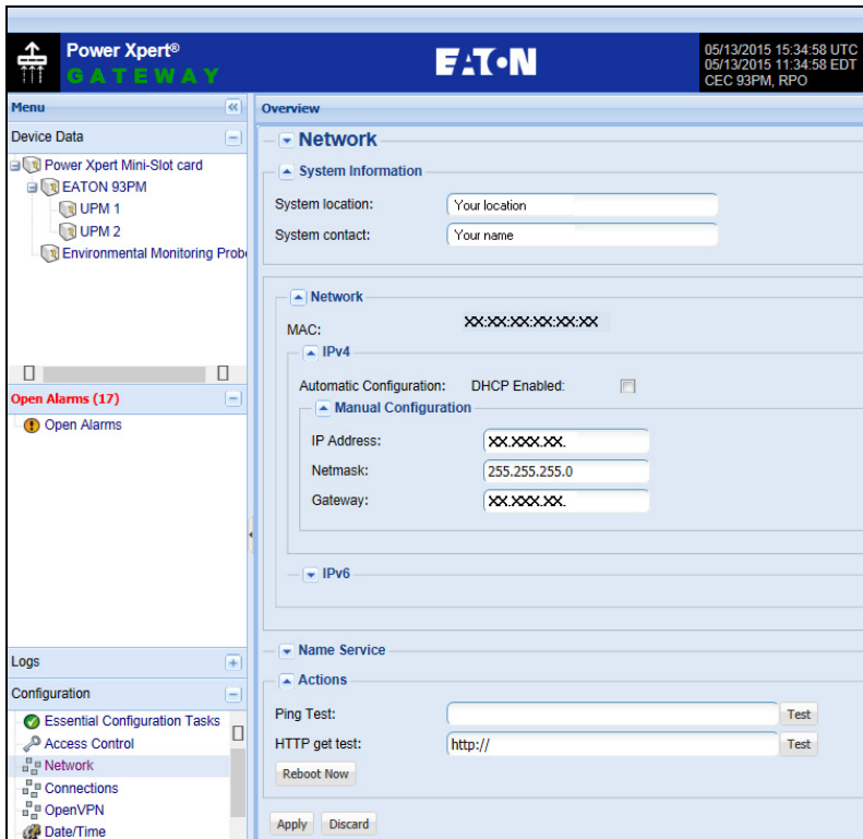
Figure 11. Disable DHCP Setting
