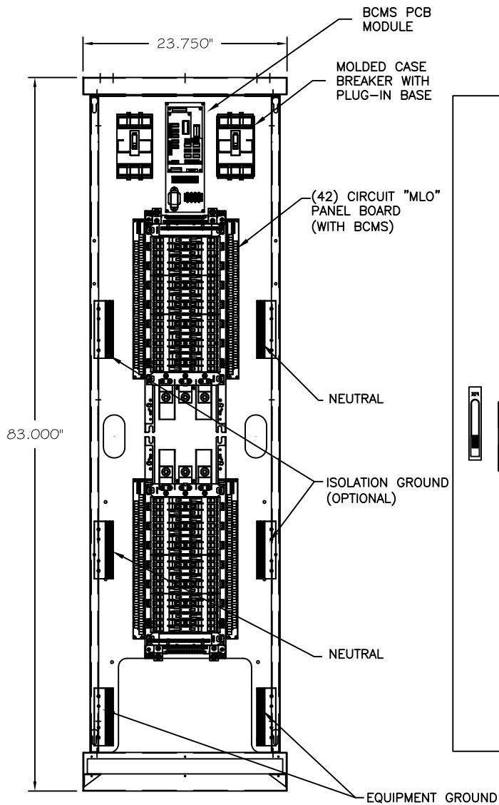
FRONT AND REAR VIEW (DOOR & COVERS REMOVED)
