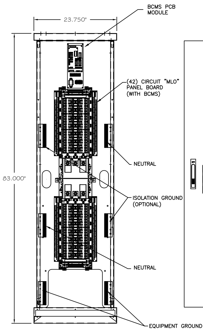
FRONT VIEW (DOOR & COVERS REMOVED)
