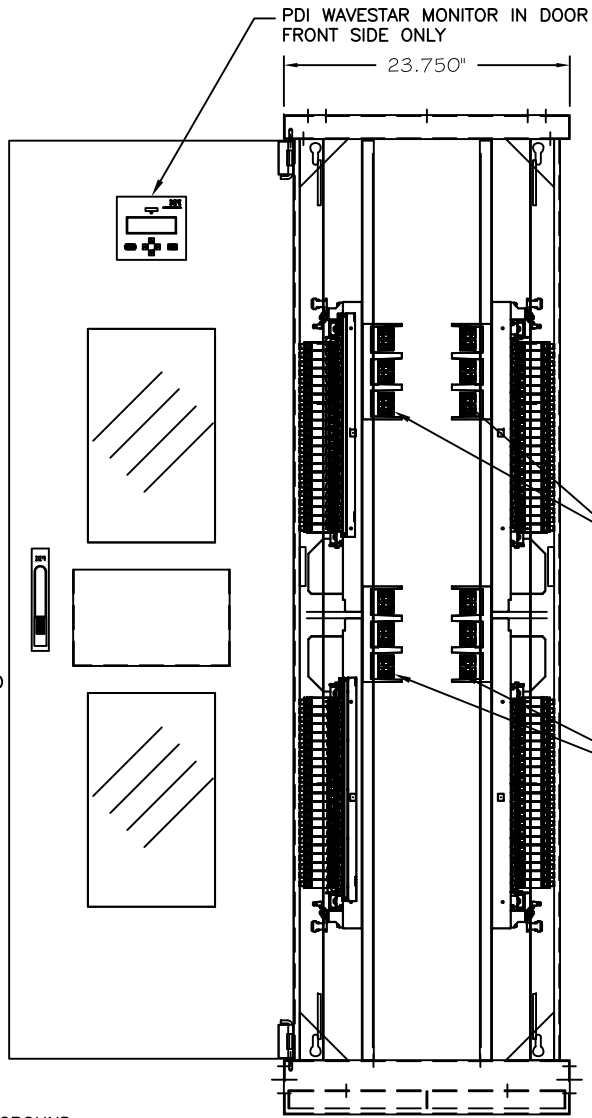
SIDE VIEW (DOOR & COVERS REMOVED)
